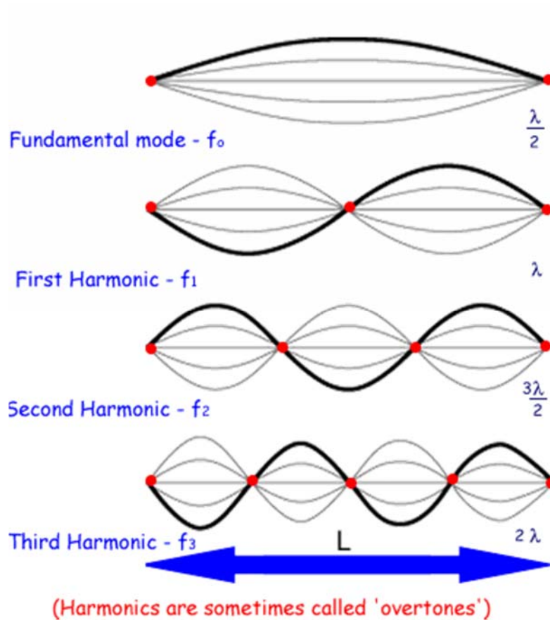
Figure 6: Standing waves corresponding to different frequencies (13).
