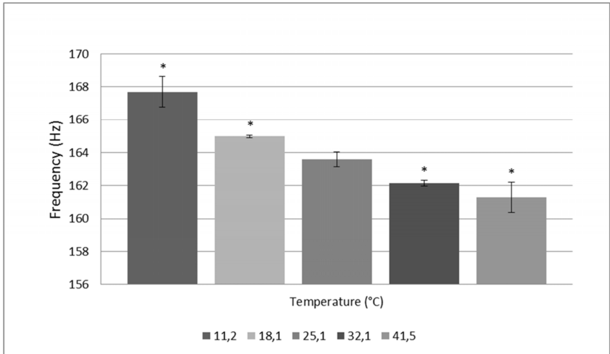
Graph 1: Guitar string frequency (Hz) changes according to the temperature(°C).
