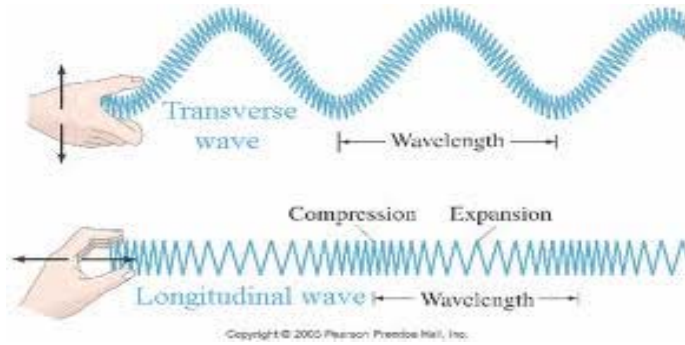
Figure 3: Transverse and longitudinal waves.
