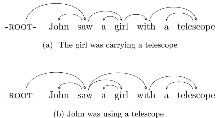
Figure 2.6: Unlabelled dependency trees that represent two different interpretation of the same sentence
