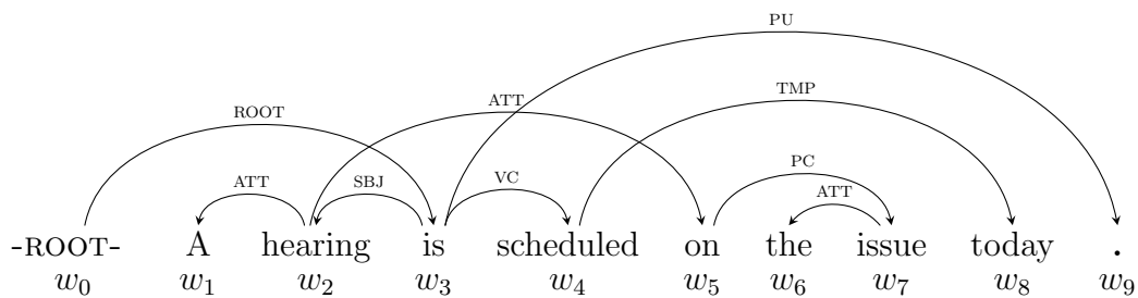
Figure 2.3: Example of dependency tree
