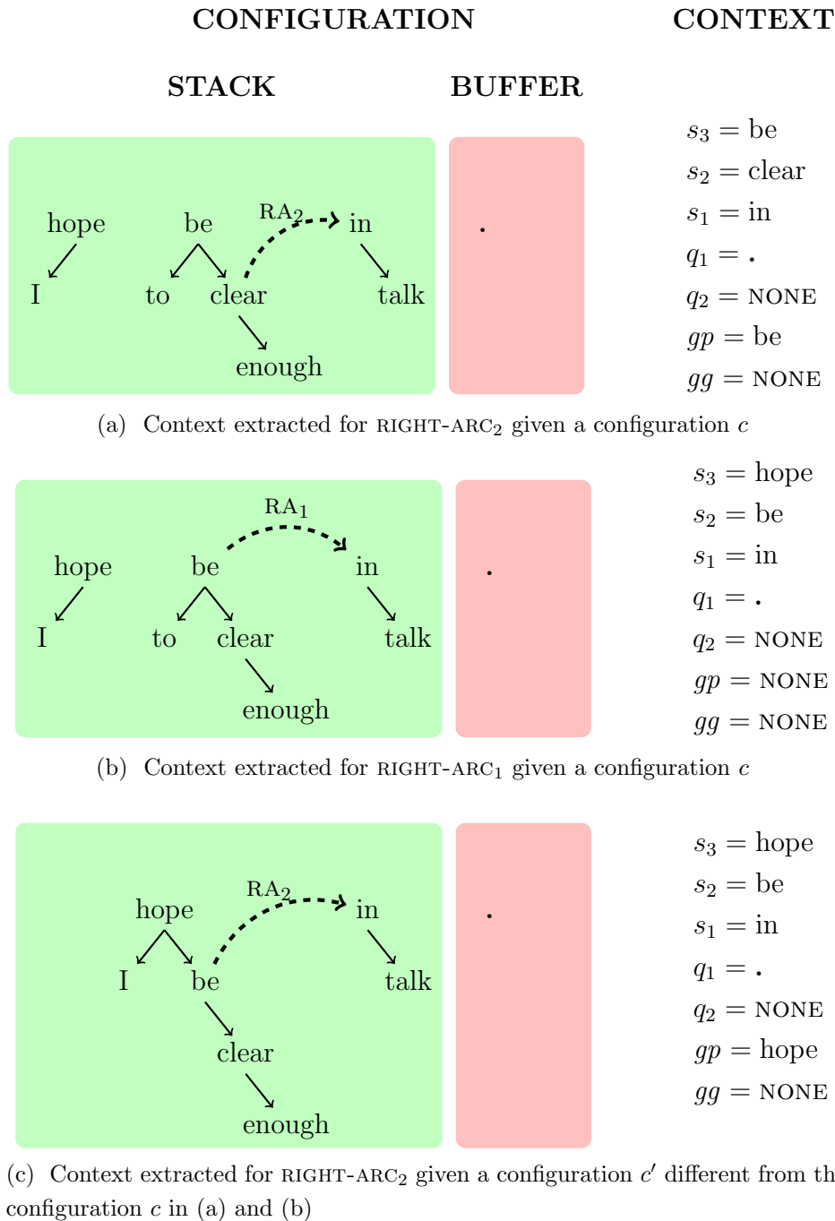
Figure 6.4: Example of context extraction for configurations that are processing the sentence s = \langle I, \text{hope}, \text{to}, \text{be}, \text{clear}, \text{enough}, \text{in}, \text{this}, \text{talk}, \cdot \rangle . In (a) and (b) we have the same configuration c but the context is extracted for a different transitions, RIGHT-ARC 2 and RIGHT-ARC 1 . In (c) we have a different configuration c' where the algorithm has already created the arc ( \text{hope} \rightarrow \text{be} ). Note that the transition and the configuration in (b) and (c) are different but the context extracted is similar because the transitions RIGHT-ARC 1 in (b) and RIGHT-ARC 2 in (c) will create the same arc ( \text{be} \rightarrow \text{in} ).
