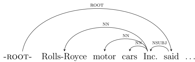
Figure 2.10: Example of dependency tree
