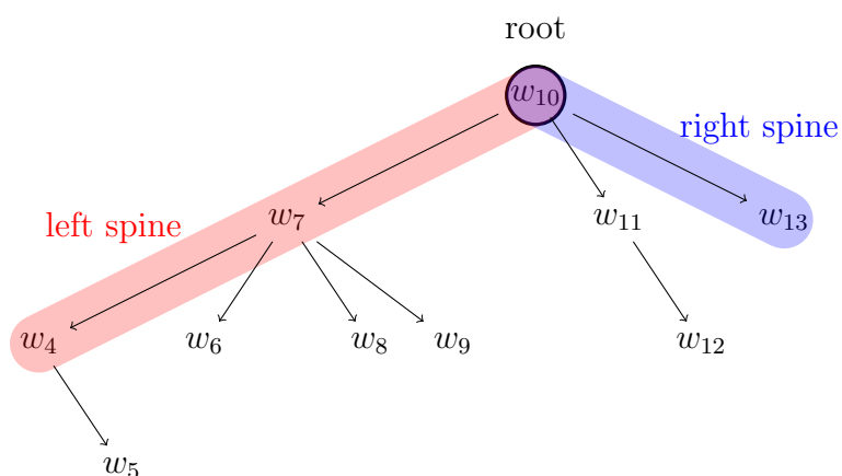
Figure 6.3: Root, Left Spine and Right Spine of a dependency tree, note that the root node belongs to both spines.
