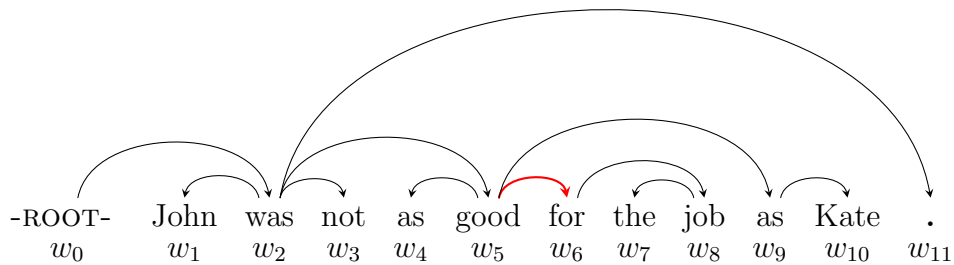
(c) Dependency tree projectivize by changing the arc w_2 \rightarrow w_6 into the arc w_2 \rightarrow w_5
