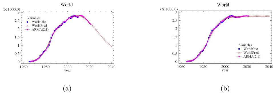
Figure 5: World nuclear power consumption: Guseo and Guidolin (2009) model and ARMA (2,1) in a life-cycle perspective (a), BM and ARMA (2,1) in a Norton-Bass perspective
