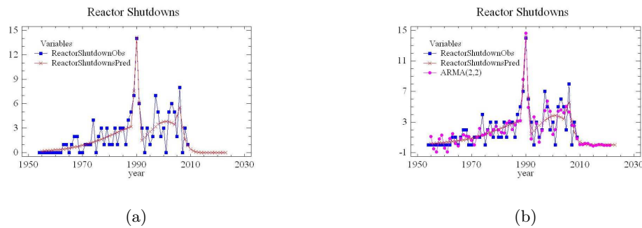
Figure 4: Dynamics of reactor shutdowns: (a) Generalized Bass model with a rectangular and an exponential shock, (b) ARMA (2,2) sharpening on autocorrelated residuals
