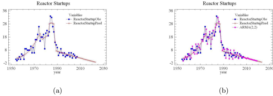
Figure 3: Dynamics of reactor startups: (a) Generalized Bass model with a rectangular and an exponential shock, (b) ARMA (2,2) sharpening on autocorrelated residuals
