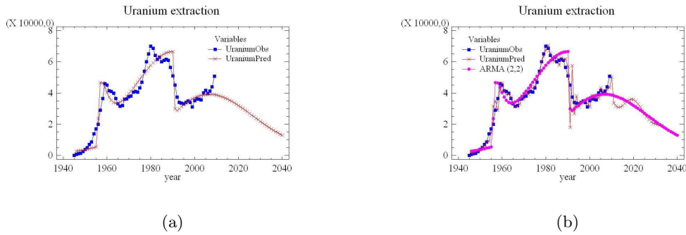
Figure 2: Dynamics of uranium extraction: (a) Generalized Bass model with two exponential shocks, (b) ARMA (2,2) sharpening on autocorrelated residuals
