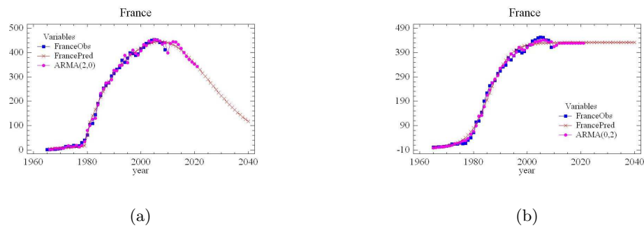
Figure 6: Nuclear power consumption in France: GBM with one exponential shock and ARMA (2,0) in a life-cycle perspective (a), BM and ARMA (0,2) in a Norton-Bass perspective
