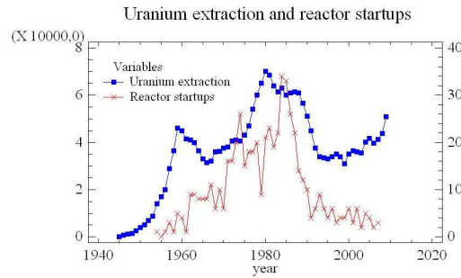
Figure 1: Dynamics of uranium extraction (in tons) and reactor startups
