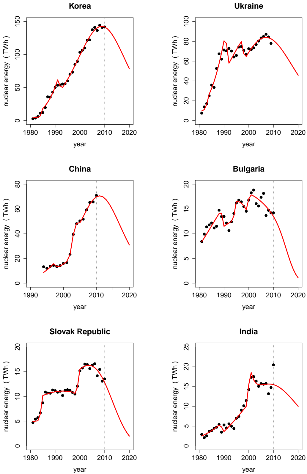
Figure 3: Annual nuclear energy (TWh) and forecasts up to 2020. Fitted models correspond to GBMs of Table 1.
