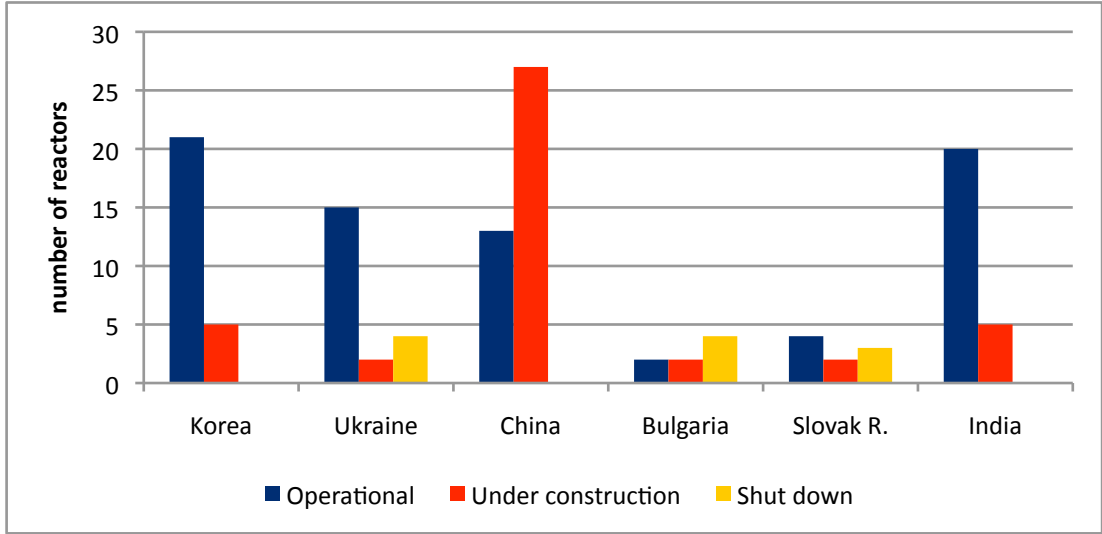
Figure 1: Number of operational, under construction, and shut-down reactors in developing countries.
