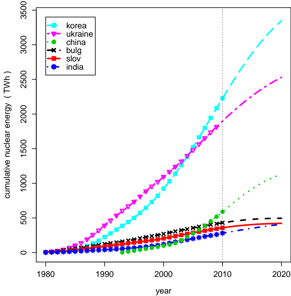
Figure 2: Observed and predicted cumulative nuclear energy (TWh). Fitted models correspond to GBMs of Table 1 and forecasts go up to 2020.
