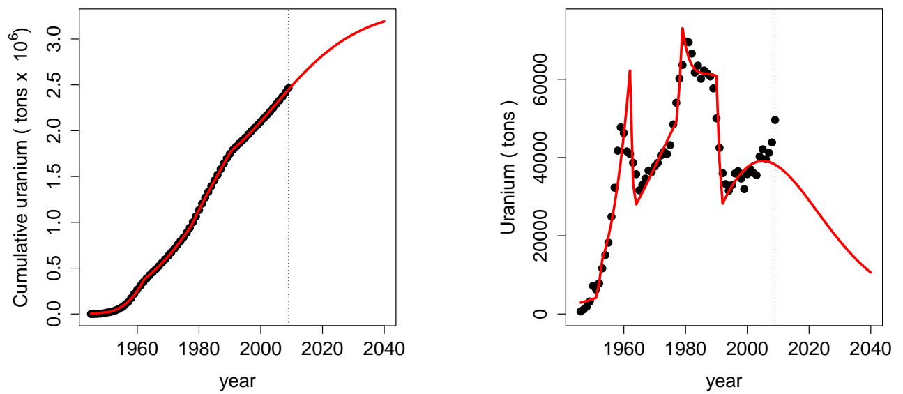
Figure 4: Cumulative annual (left panel) and annual (right panel) uranium world extraction (tons) and forecasts up to 2040 (Table 1).
