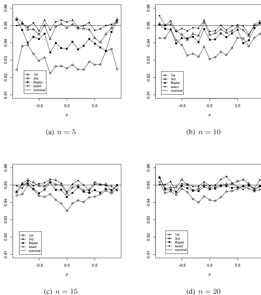
Figure 3: Simulation 1: bivariate normal with means 0 and variances 1. Empirical coverage of nominal two-sided 95% confidence intervals for \gamma for varying values of \rho and sample sizes n = 5, 10, 15, 20 . Pivots used: likelihood root r (1st), modified likelihood root r^* (3rd); Bayesian modified likelihood root r_B^* (Bayes); expression (14) by Haddad and Provost (2011) (exact). Based on 10,000 replicates.
