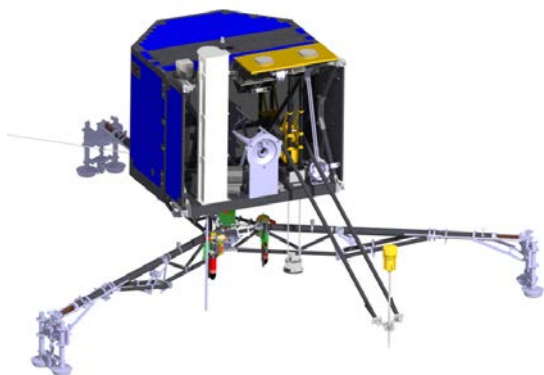
Figure: Illustration of Philae with deployed landing gear and instruments [1]
