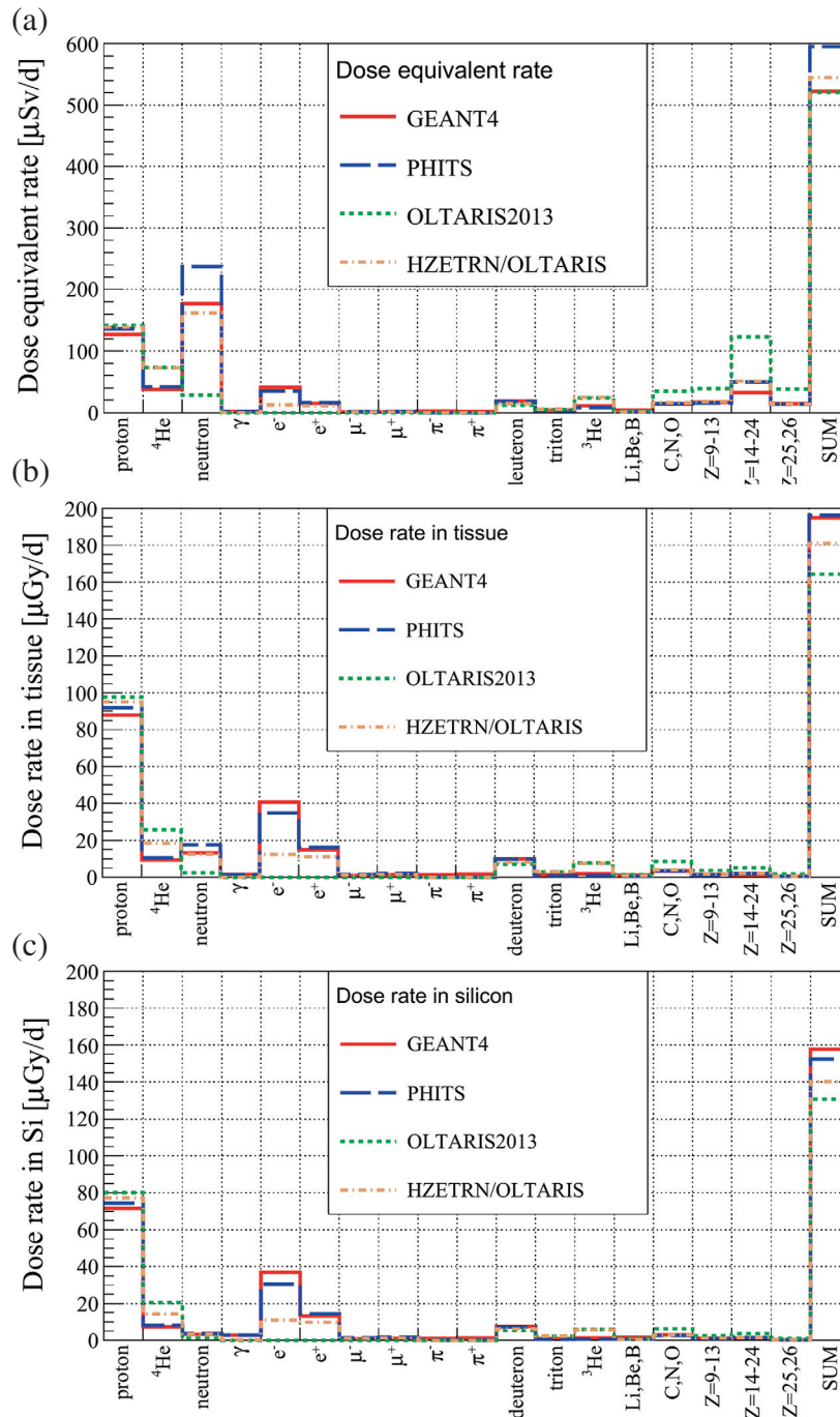
Fig. 11. Contribution of different particle types to the dose equivalent rate in tissue (a, in \mu\text{Sv/d} ), dose rates (in \mu\text{Gy/d} ) in tissue (b), and silicon (c) calculated with different transport models for the Martian surface (atmospheric shielding: 22 \text{ g/cm}^2 ). MSL-RAD measured a dose rate in tissue of 0.21 \pm 0.04 \text{ mGy/day} and a dose equivalent rate of 0.64 \pm 0.12 \text{ mSv/day} Hassler et al. 2014).
