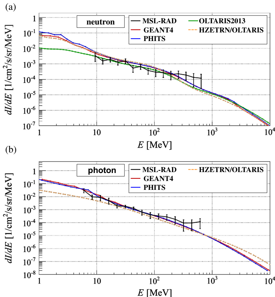
Fig. 4. Neutral particle spectra (all incident angles) on the Martian surface measured between 19 August 2012 and 17 February 2013 by MSL-RAD (black, Köhler et al. 2014) and calculated for the same period by different simulation tools: GEANT4 (red), PHITS (blue), OLTARIS2013 (green), HZETRN/OLTARIS (ocher).
