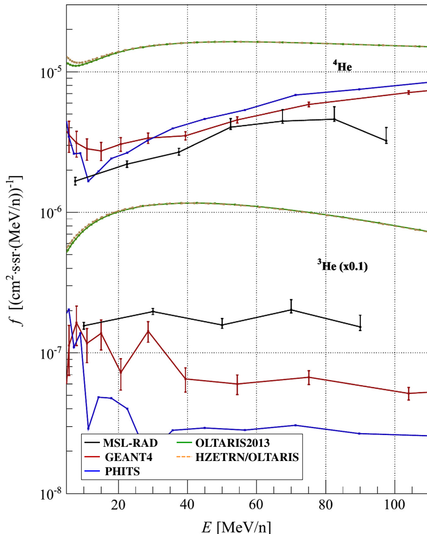
Fig. 6. ^4\text{He} and ^3\text{He} (scaled by 0.1) spectra for zenith angles smaller than 30^\circ on the Martian surface measured between 19 August 2012 and 17 February 2013 by MSL-RAD (black, Ehresmann et al. 2014) and calculated for the same period by different simulation tools: GEANT4 (red), PHITS (blue), OLTARIS2013 (green), HZETRN/OLTARIS (ocher). The data have been scaled by the factors given in parentheses.
