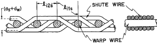
Fig. 1. Cross-sectional views of plain weave (plain square, full twill, and fourdrinier) and dutch weave (plain dutch and twilled dutch) screens.
