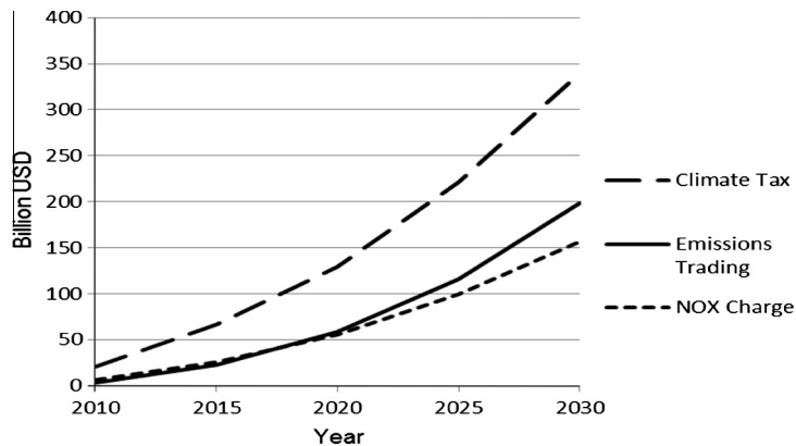
Fig. 5. Costs of different market-based measures analysed in Scenario “World”, assuming the ‘High Price Path’ and the metric atr 50 . The costs are scaled to 2012 prices. The measure “NO x Charge” includes CO 2 trading and operational measures (flying lower).
