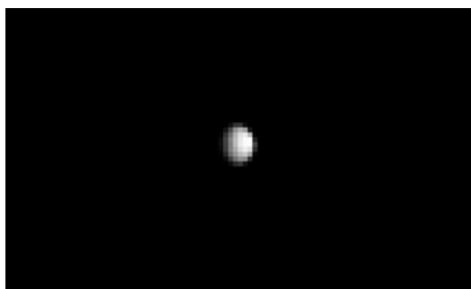
Figure 1. Ceres imaged by Dawn on December 1, 2014 at a distance of about 10^6 km
