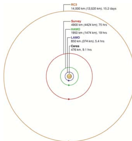
Figure 2. Science orbits used at Ceres
