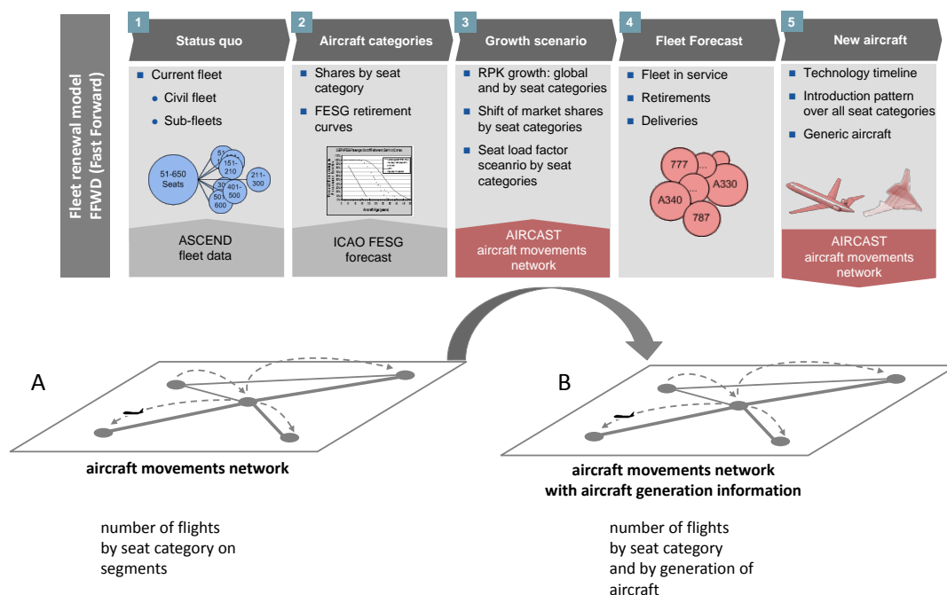
Figure 6: Forecasting an aircraft movements network with aircraft generation information: Interfaces between the aircraft movements layer and the fleet renewal model FFWD [3]
