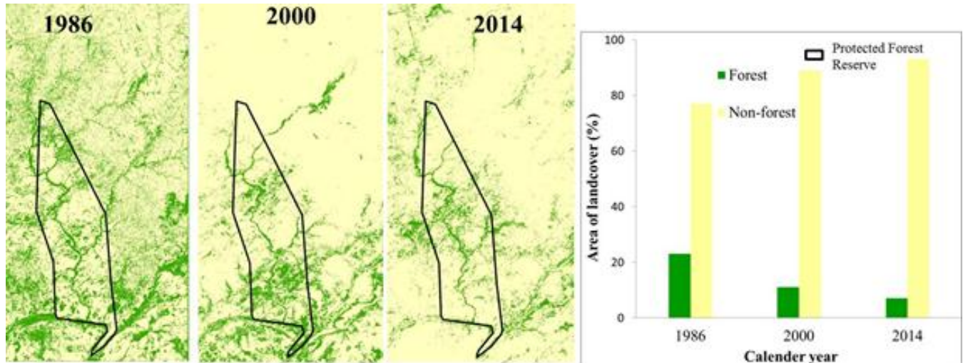
Figure 2. Landcover in the headwaters of Tankwidi river basin for the studied years (1986-2014).
