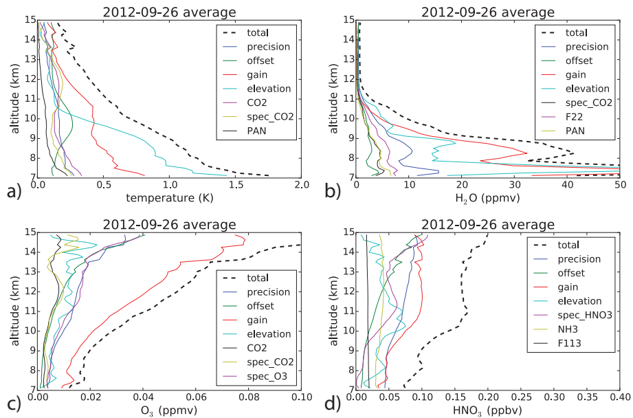
Figure 4. Total error and major error sources for the four primary targets temperature (a), H 2 O (b), O 3 (c), and HNO 3 (d) averaged over the profiles of the flight of 26 September 2012. A “spec” prefix notes the error induced by spectral uncertainty of line intensities.
