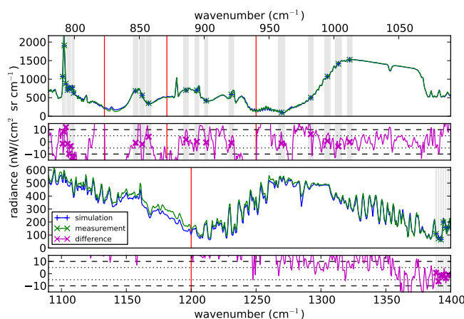
Figure 3. A measured and a simulated dynamics mode spectrum averaged over row 57 (tangent altitude 12.78 km) of the detector taken at 14:40:12 UTC and 14.45 km aircraft altitude. The spectrum is split at 1090 \text{cm}^{-1} with the lower panels showing higher wavenumbers. The lines show the full spectral resolution of the spectra while the markers show the values of the ISWs used in the retrieval. The extent of the ISWs is overlaid as grey bars. The difference plots also contain the target (dots) and threshold (dashes) values for noise. The vertical red lines separate regions that employ different aerosol/extinction profiles. This simulation was performed using the band model. The large discrepancy in the lower panels is caused by \text{N}_2\text{O} and \text{CH}_4 , which are currently not retrieval targets.
