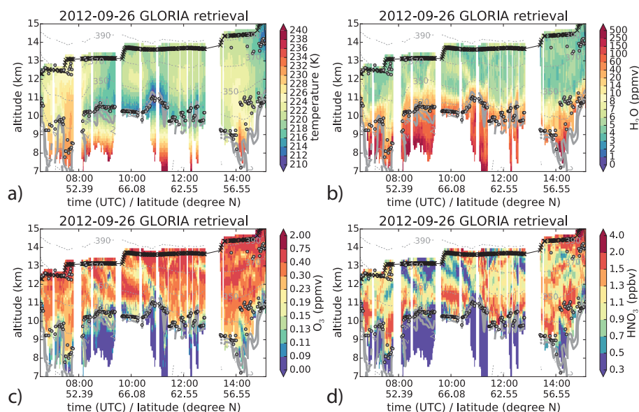
Figure 6. Cross-sections of retrieved quantities for the flight of 26 September 2012: temperature (a), H 2 O (b), O 3 (c), and HNO 3 (d). In addition, selected isentropes are shown as dotted grey lines, ECMWF potential vorticity (interpolated to the time of measurement) isolines of 2 and 4 PVU are shown as thick grey lines. The thermal tropopause is derived from retrieved temperature profiles and is shown as thick grey dots. Depicted retrieved values are limited below by clouds and above by the flight altitude.
