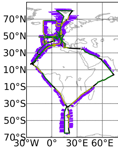
Figure 1. Overview over the flights performed during TACTS and ESMVAL. The flight paths are marked as black lines. Atmosphere measurements of GLORIA are overlaid in dark and light green for chemistry and dynamics mode, respectively. The tangent points of preliminarily processed profiles are shown in blue.
