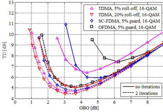
(c) TD of 16-QAM.
