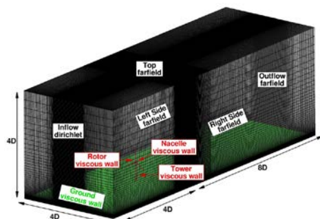
(a) Dimensions and boundary conditions for the simulation of the complete turbine
