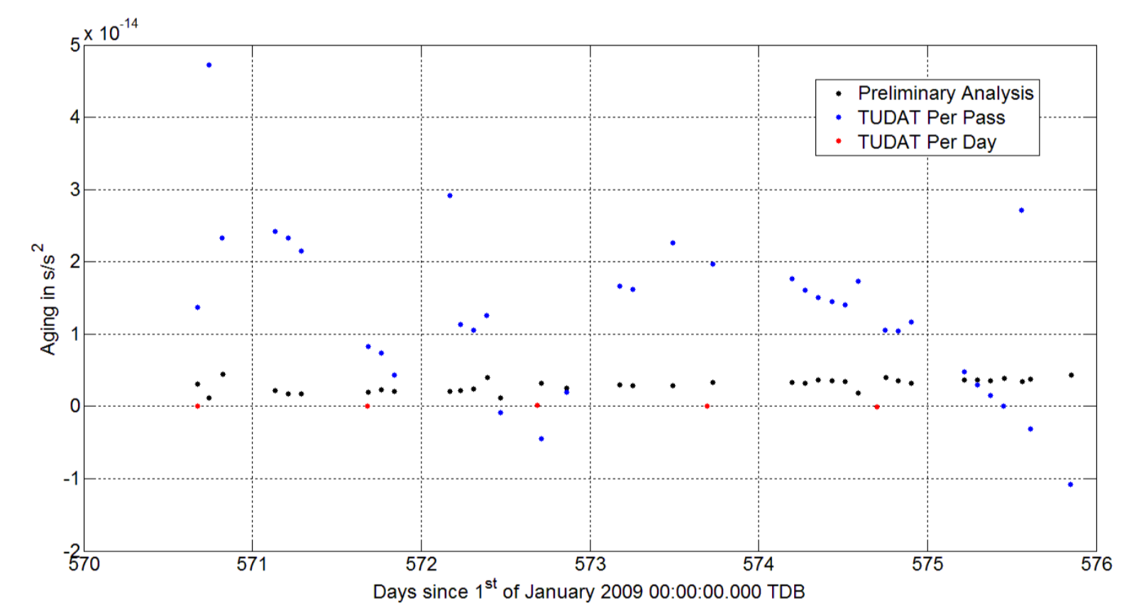
Figure 5: Estimated aging values
