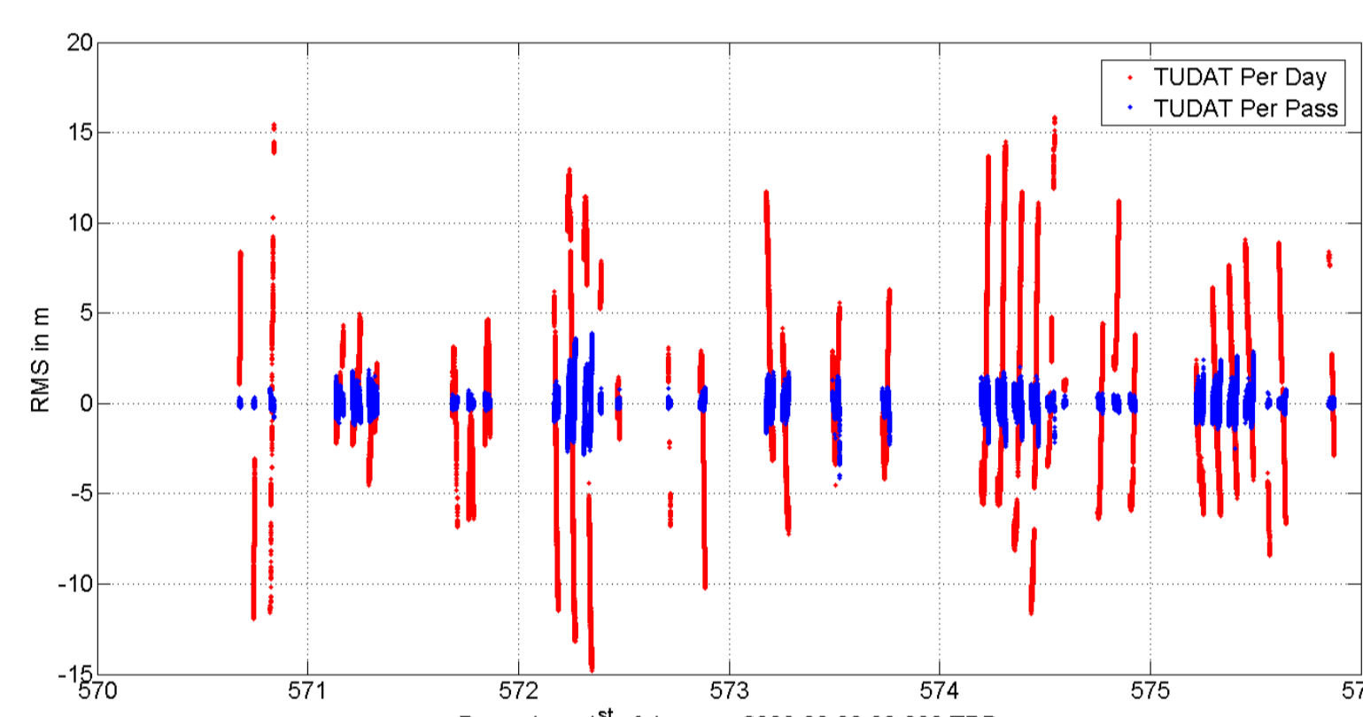
Figure 3: RMS of the measurements w.r.t. the derived trajectory
