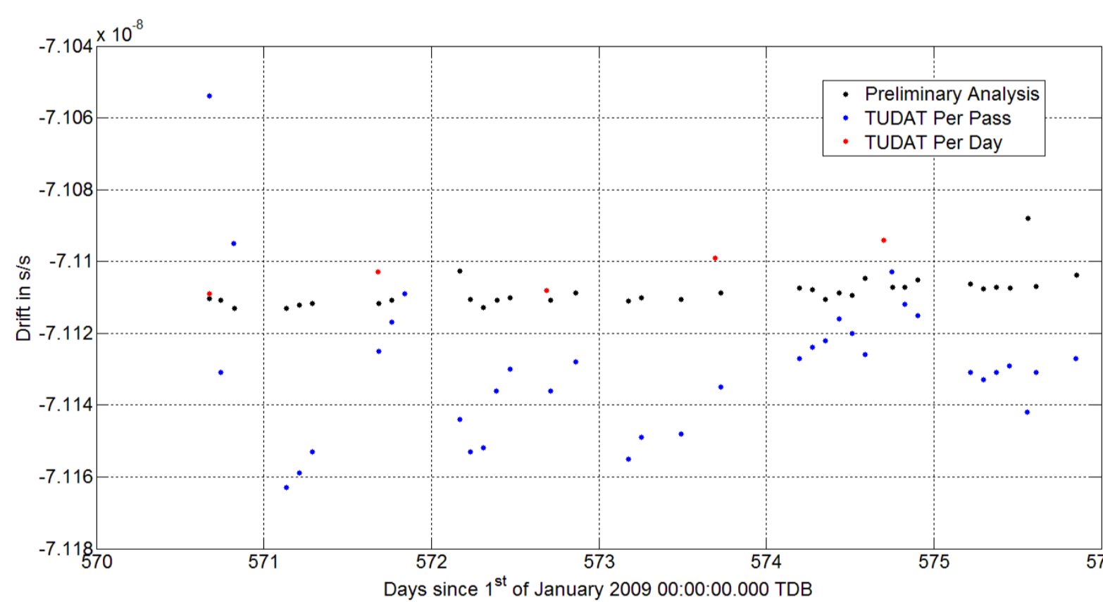
Figure 4: Estimated drift values
