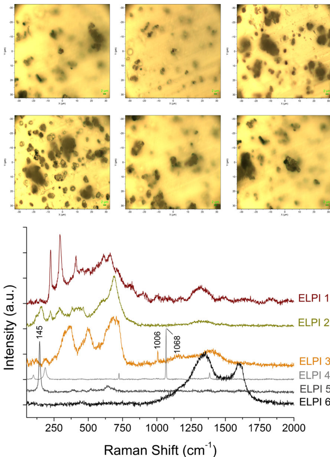
Fig. 3 Optical microscope images and corresponding Raman spectra of the aerosol particles (ELPI) collected with the ELPI, Munich from April 16 to 19, 2010. The spectra were collected at the positions x=0, y=0
