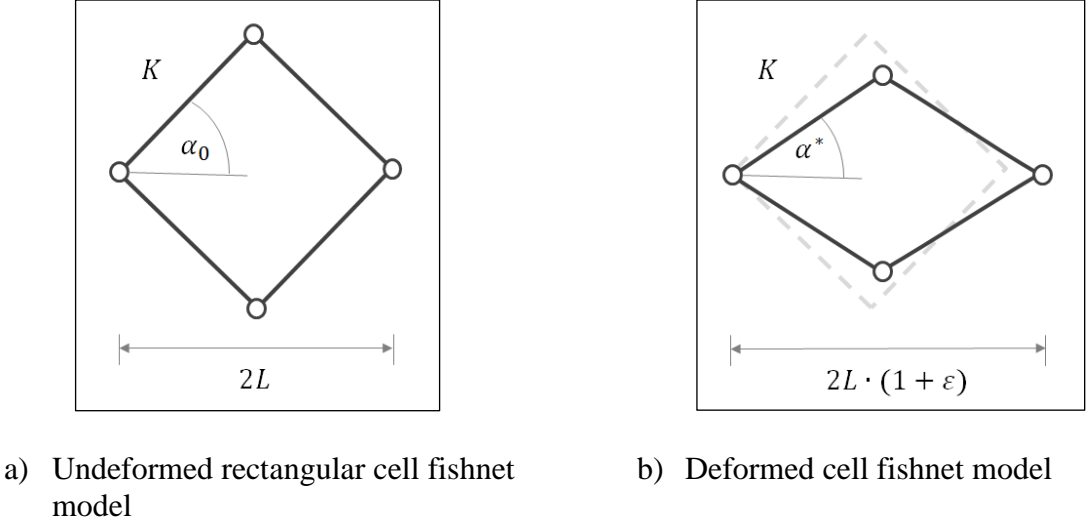
Figure 13: Fishnet model of a textile material
