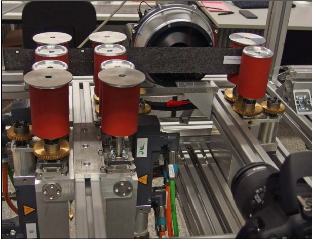
Figure 14. Elongation test setup
