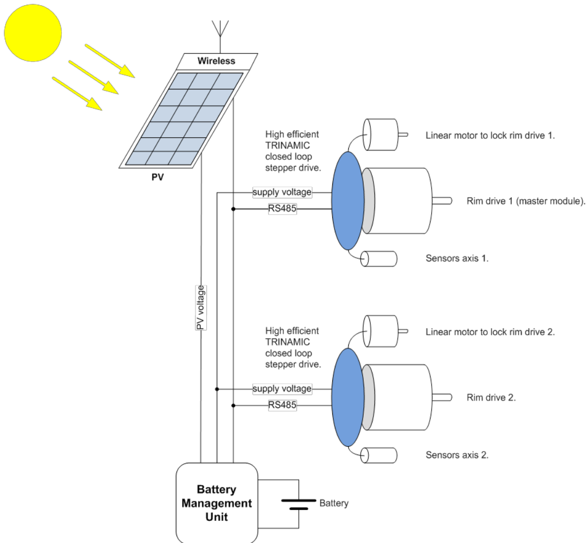
Fig. 2. Rim drive heliostat electrical system architecture.
