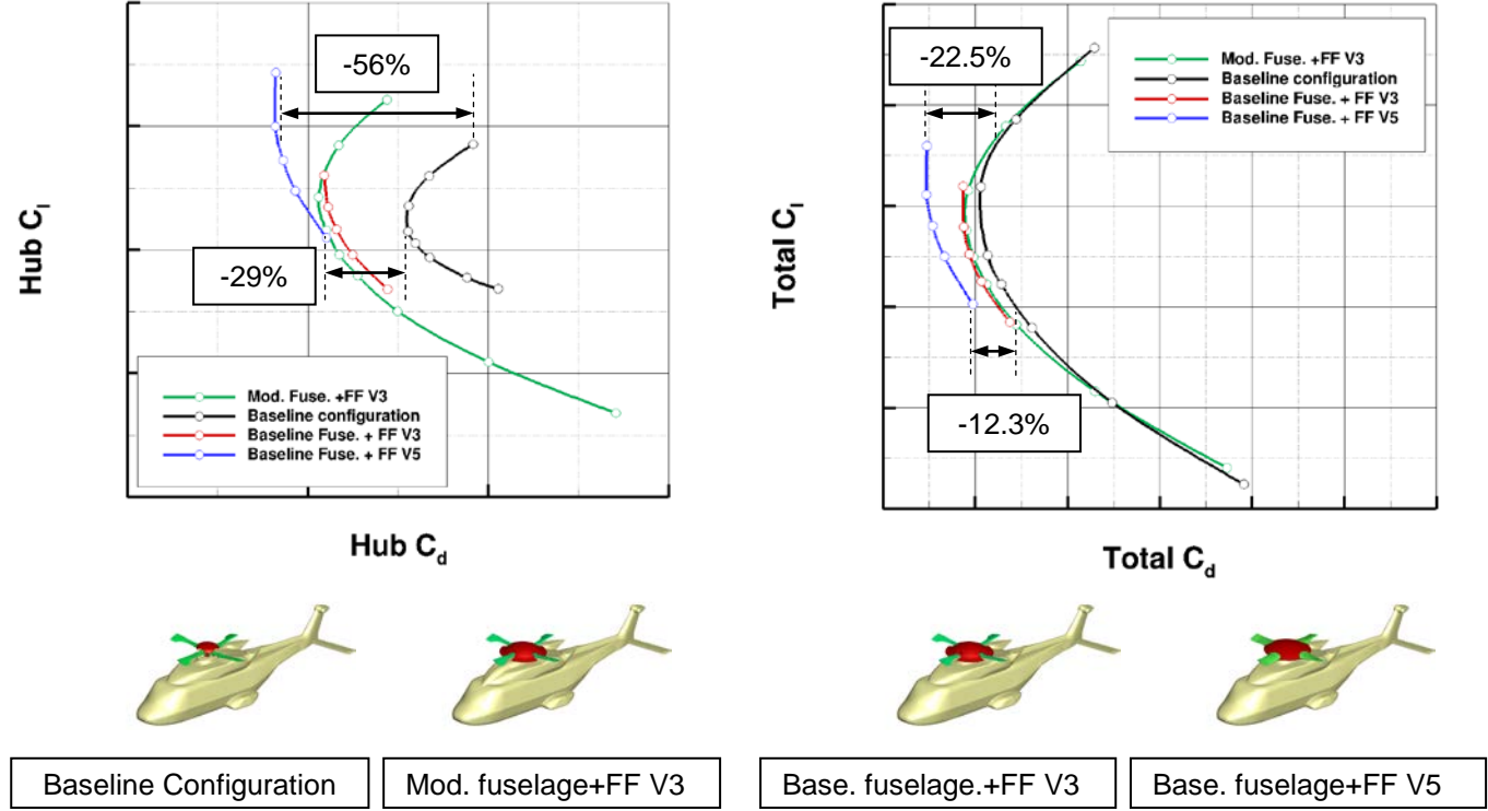
Figure 10: Drag-lift polars for the hub (left), and the complete configuration (right) for different configurations in free stream conditions at cruise Mach number Ma=0.204
