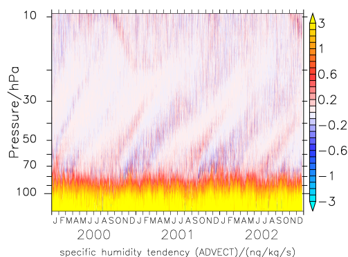
Figure 9. Time series of the average over the 5° S–5° N latitudinal band of the advection tendency (in \text{ng kg}^{-1} \text{s}^{-1} ) of the specific humidity.
