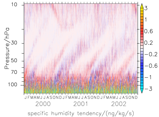
Figure 4. Time series of the average over the 5° S–5° N latitudinal band of the total tendency (in \text{ng kg}^{-1} \text{s}^{-1} ) of the specific humidity.
