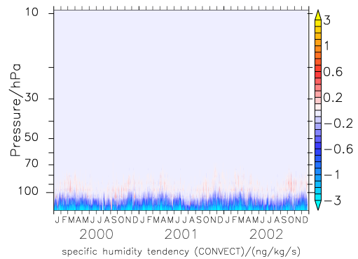
Figure 6. Time series of the average over the 5° S–5° N latitudinal band of the convective cloud tendency (in \text{ng kg}^{-1} \text{s}^{-1} ) of the specific humidity.
