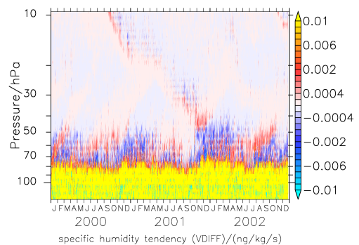
Figure 7. Time series of the average over the 5° S–5° N latitudinal band of the vertical diffusion tendency (in \text{ng kg}^{-1} \text{s}^{-1} ) of the specific humidity.
