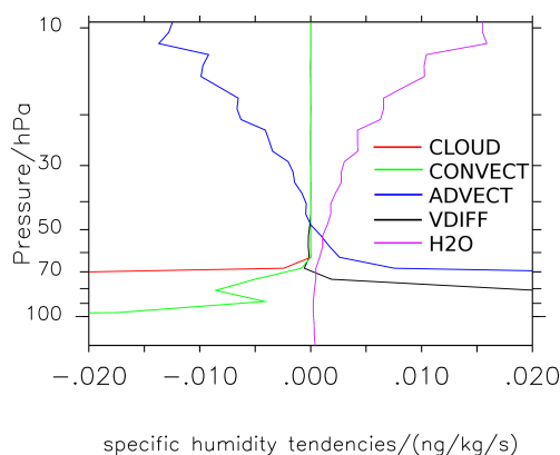
Figure 10. Zonally averaged process tendencies of the specific humidity (in \text{ng kg}^{-1} \text{s}^{-1} ) at the Equator, averaged over the 3-year time period.
