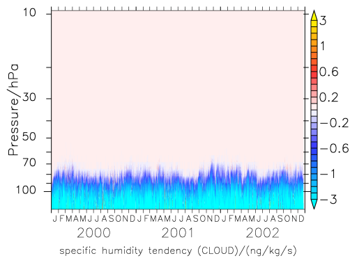
Figure 5. Time series of the average over the 5° S–5° N latitudinal band of the large-scale cloud tendency (in \text{ng kg}^{-1} \text{s}^{-1} ) of the specific humidity.
