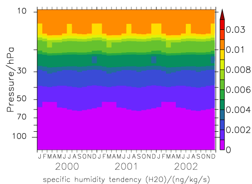
Figure 8. Time series of the average over the 5° S–5° N latitudinal band of the methane oxidation tendency (in \text{ng kg}^{-1} \text{s}^{-1} ) of the specific humidity.
