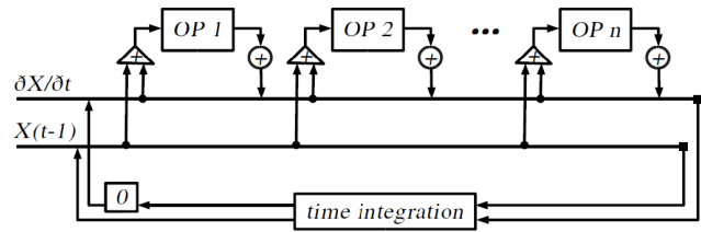
Figure 1. Operator splitting concept (image taken from Jöckel et al., 2005). For explanation see text.
