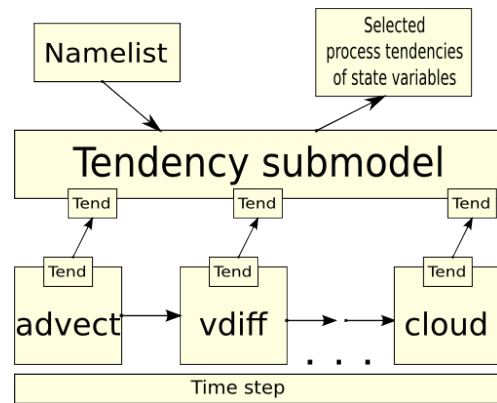
Figure 2. Schematic of the MESSy TENDENCY submodel within the framework of the EMAC model system. The addition of the individual process tendencies to the total tendency is now outsourced from the respective submodels to the TENDENCY submodel. A user-controlled namelist provides several possibilities for the output of the process tendencies of state variables.
