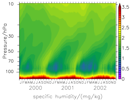
Figure 3. Time series of the average over the 5° S–5° N latitudinal band of the specific humidity (in \text{mg kg}^{-1} ).
