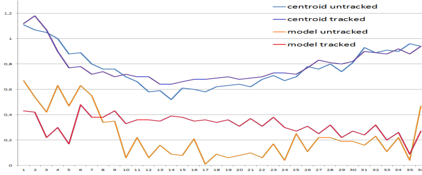
Figure 6: Position errors, scene 3 (50 km/h)
