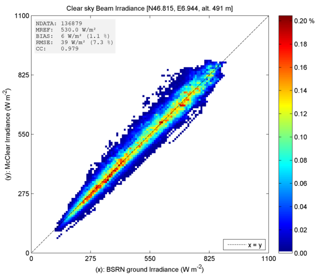
Fig. 5. Scatter density plot between BSRN 1 min clear-sky data and McCClear. Payerne. Beam irradiance on horizontal surface.
