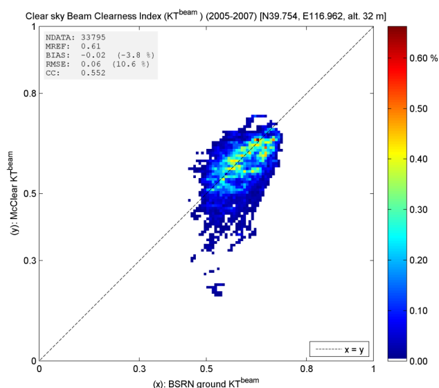
Fig. 11. Scatter density plot between BSRN 1 min clear-sky data and McClear. Xianghe. Beam clearness index KT^{dir} .
