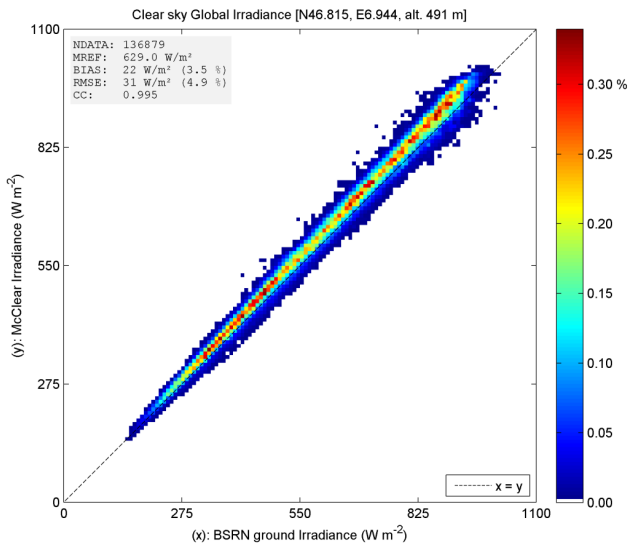
Fig. 4. Scatter density plot between BSRN 1 min clear-sky data and McCClear. Payerne. Global irradiance on horizontal surface.
