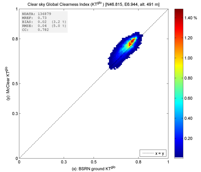
Fig. 6. Scatter density plot between BSRN 1 min clear-sky data and McCClear. Payerne. Global clearness index KT.
