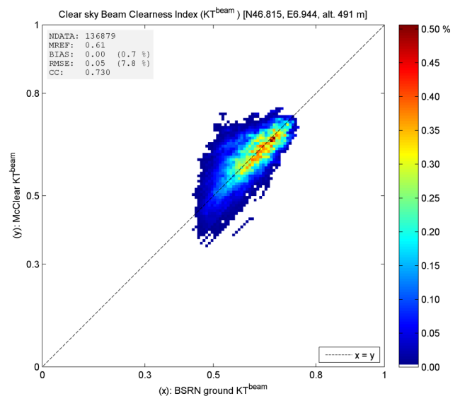
Fig. 7. Scatter density plot between BSRN 1 min clear-sky data and McCClear. Payerne. Beam clearness index KT dir .
