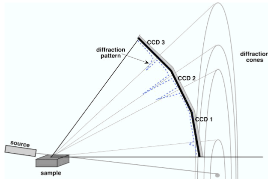
Figure 1: Reference diffraction geometry of Mars-XRD.
