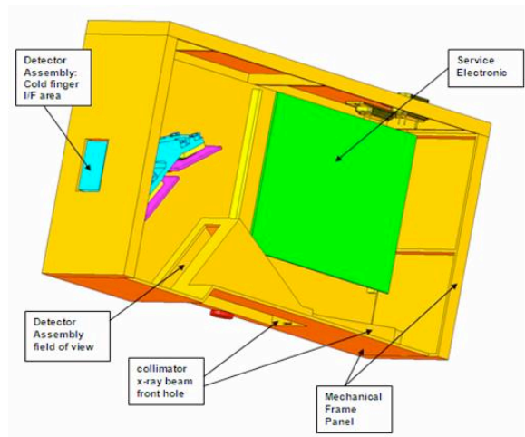
Figure 2: Drawing of the Mars-XRD flight model.
