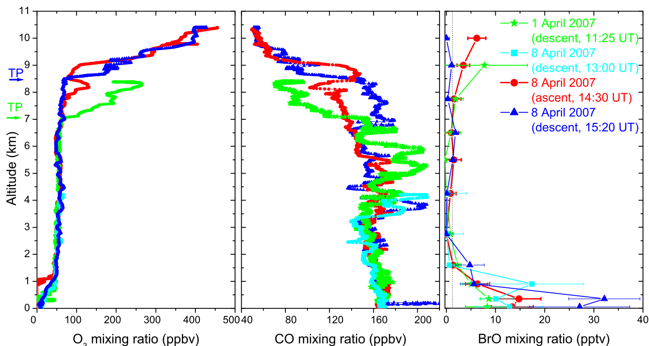
Fig. 9. Aircraft-borne measurements performed by the DLR ( \text{O}_3 and CO) and the IUP-HD group (BrO) on 1 April (green) and 8 (cyan, red, blue) during the ASTAR 2007 campaign. Note that the maximum altitude in the cyan profiles (descent at 13:00 UT, 8 April) is around 4 km. The tropopause height for 1 April (green) and 8 (blue) are indicated with arrows in the left panel. Further details of both sorties are given in Prados-Roman (2010). The dashed vertical line on the right panel indicates the BrO detection limit.
