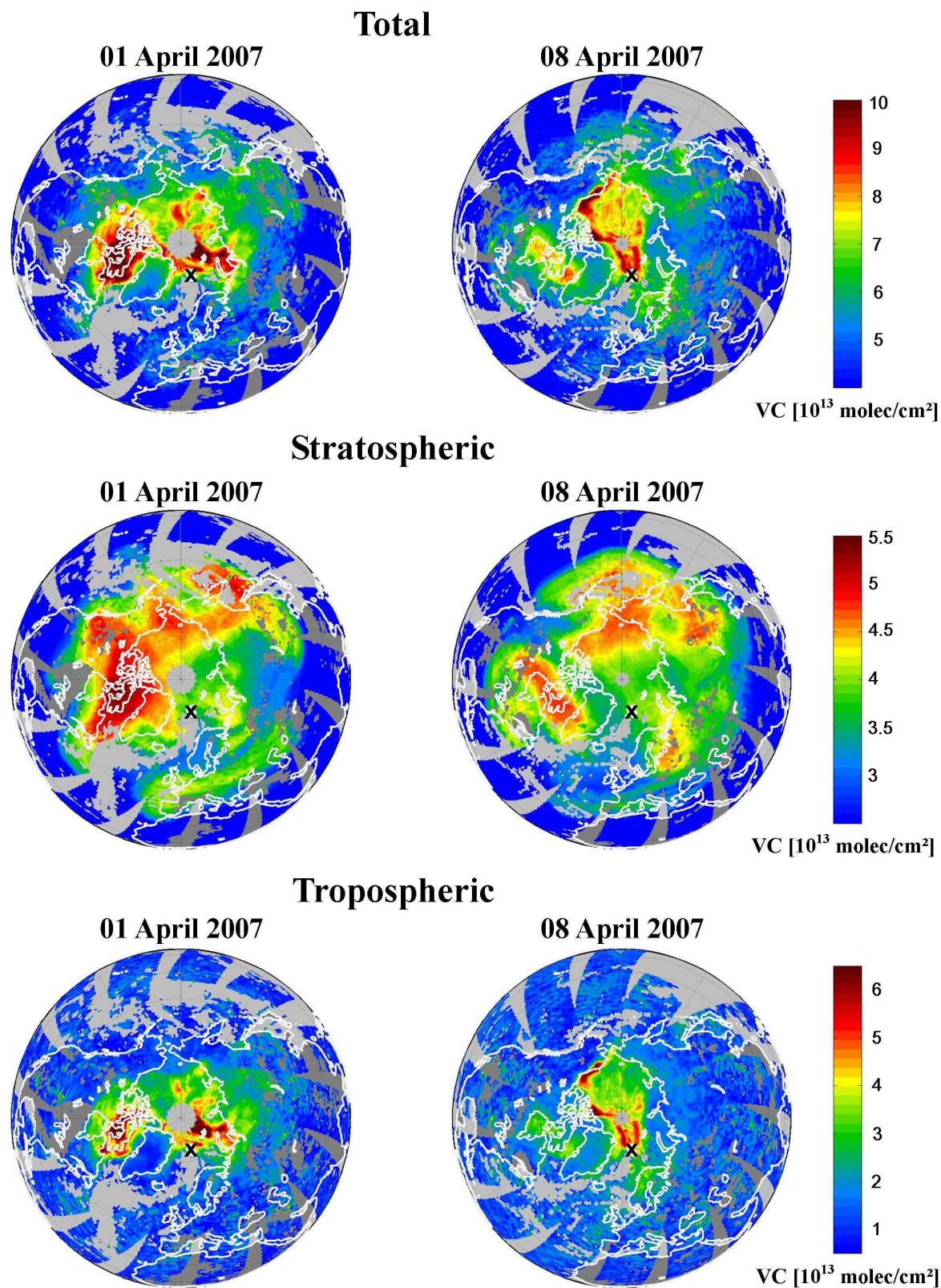
Fig. 10. GOME-2 total (upper panels), stratospheric (middle panels) and tropospheric (low panels) BrO Vertical Column Densities for the 1 and 8 April 2007 (left and right column, resp.). The island of Spitsbergen, base of the ASTAR 2007 campaign, is marked with black crosses. Details of the retrieval method are given in Theys et al. (2011).
