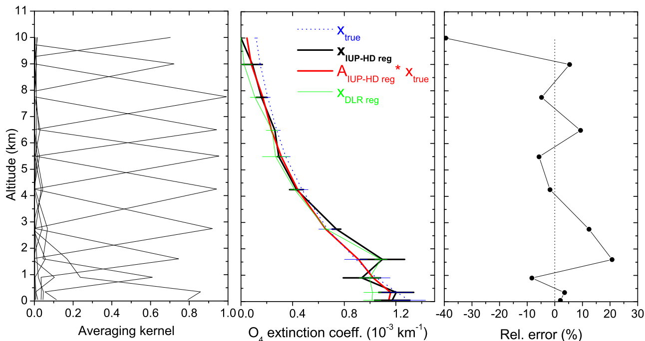
Fig. 7. Retrieval of the vertical distribution of the \mathcal{E}_{\text{O}_4} . Left: Averaging kernels showing \sim 8 degrees of freedom. Center: The \mathcal{E}_{\text{O}_4} true state is shown in blue (considering 10% error). X_{\text{IUP-HD reg}} (in black) is the regularized \mathcal{E}_{\text{O}_4} profile if the IUP-HD \mathcal{E}_{\mathcal{M}} profile (see Fig. 5) is included in the RT model (the error bars include the retrieval noise and the effect of uncertainties of the ground albedo and the aerosol load). The contribution of the true state to the row space (IUP-HD reg) is shown in red. For comparison purposes, X_{\text{DLR reg}} (in green) corresponds to the regularized \mathcal{E}_{\text{O}_4} profile if DLR \mathcal{E}_{\mathcal{M}} (b) profile (in dark blue in Fig. 5) is included in the RT model. Right: Relative error of the (IUP-HD) \mathcal{E}_{\text{O}_4} retrieval.
