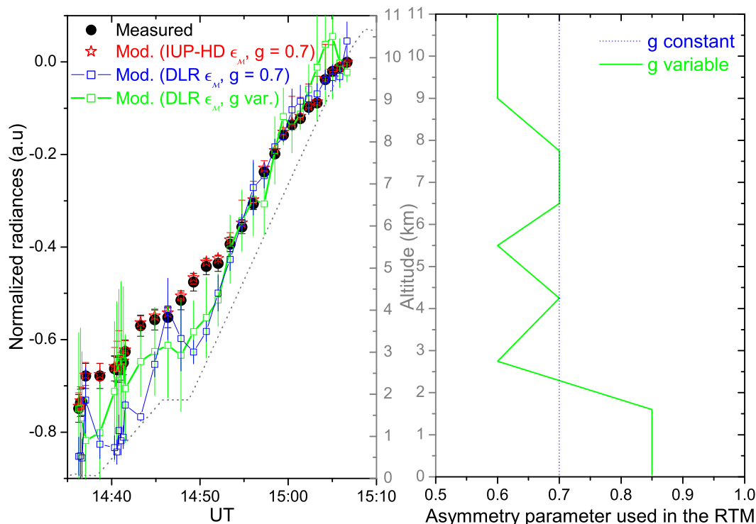
Fig. 6. (Left) Sun normalized radiances measured and modeled during the 14:30 UT ascent (the dotted line represents the flight track). Measured radiances (at 353 nm) are shown in black. At 353 nm and 79 % ground albedo, radiances are modeled considering different \mathcal{E}_{\mathcal{M}} (refer to Fig. 5) and asymmetry parameter scenarios. Red: IUP-HD \mathcal{E}_{\mathcal{M}} with g = 0.7 . Blue: DLR \mathcal{E}_{\mathcal{M}} with g = 0.7 . Green: DLR \mathcal{E}_{\mathcal{M}} with variable g . Error bars of all modeled radiances include their wavelength dependency (349–360.8 nm). In addition, a ground albedo uncertainty of 20 % is considered for the DLR radiances. (Right) Profiles of the aerosol asymmetry parameter considered for the RT studies ( g within the range of 0.6–0.85 as reported for the Arctic, e.g., Lampert et al., 2009).
