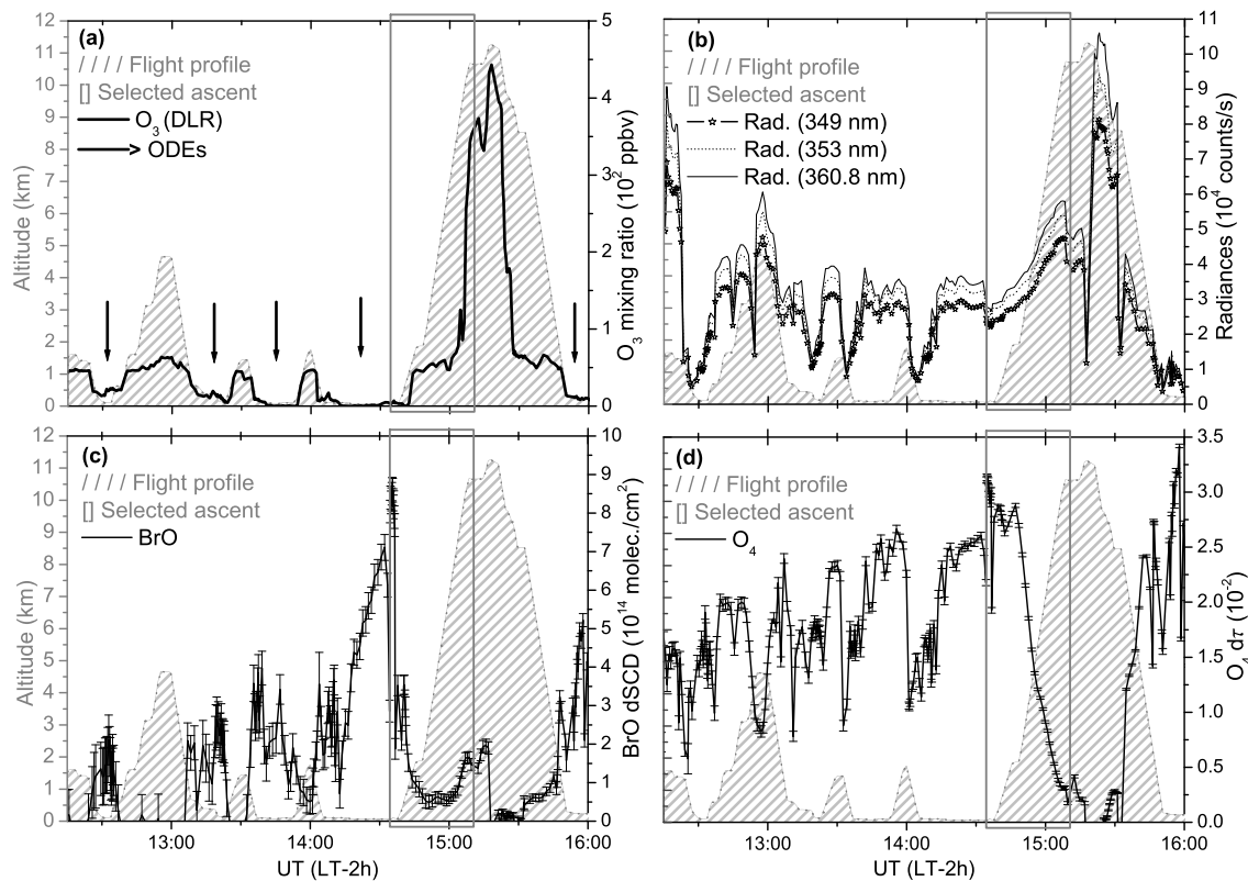
Fig. 1. Measurement flight on 8 April 2007 (72–80°SZA). Panel (a) shows the O 3 mixing ratios measured in situ with an UV absorption photometer (DLR). Flight sections within the Arctic BL with ODEs are indicated by arrows. Panels (b)–(d) show, resp., the radiances at different wavelengths, the BrO dSCDs and the O 4 d\tau measured with the UV channel of the mini-DOAS instrument. The tropospheric vertical profiles of the aerosols \mathcal{E}_M and of the trace gases presented in this work are retrieved from data measured during the aircraft ascent starting at around 14:30 UT (box).
