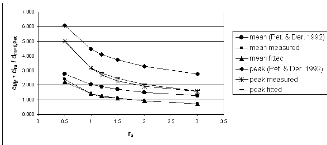
Figure 20: c_{My} \cdot d_{ra} / d_{ra=1, Pet} at load case 1
