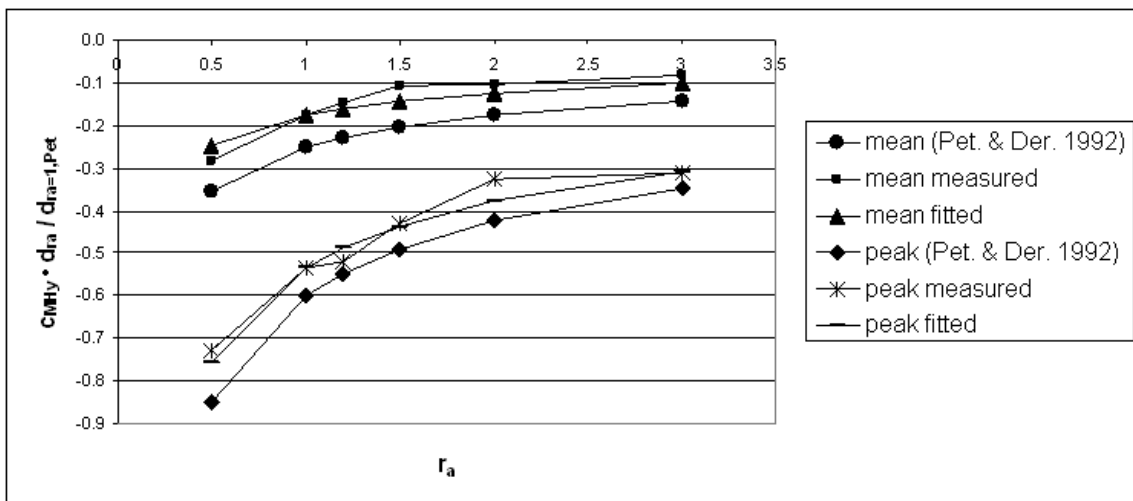
Figure 17: cM_{Hy} \cdot d_{ra} / d_{ra=1,Pet} at load case 2
