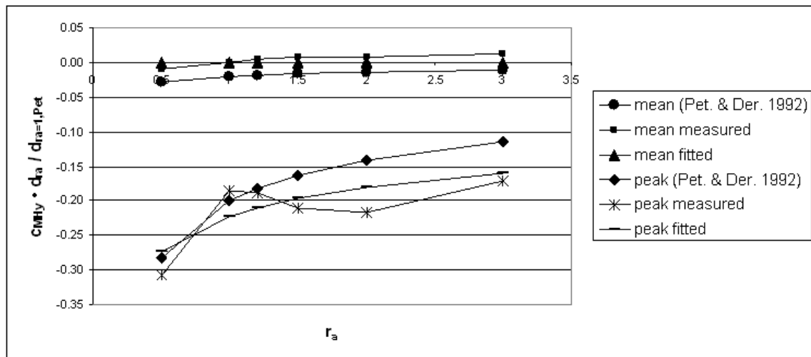
Figure 19: c_{MHy} \cdot d_{ra} / d_{ra=1,Pet} at load case 4
