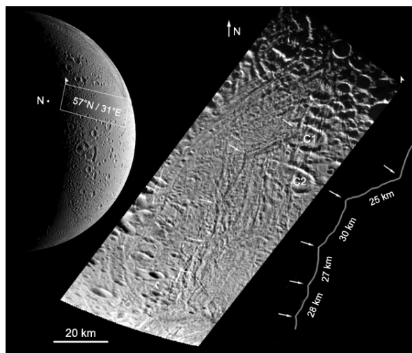
Fig. 2: NE-SW trending arcuate segments and cusped features (arrows) located at northern latitudes. Note that these segments formed in a weak icy lithosphere which is suggested by two highly-strained craters (c1, c2) in this area.
