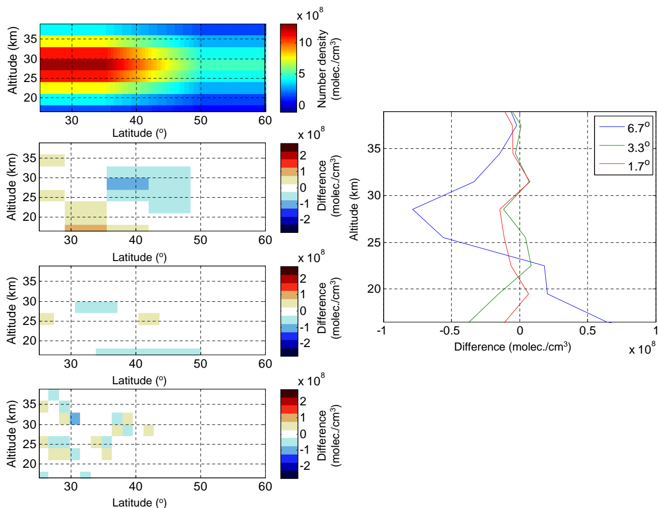
Fig. 14. 2-D retrieval for different distances between consecutive scanning sequences. On the left: the \text{NO}_2 field of the simulation (top) and the differences between the retrieved number density and the true values with the distance of 6.7^\circ (second plot), 3.3^\circ (third plot) and 1.7^\circ (bottom plot). On the right: mean differences are plotted for the southern part of the gradient (i.e. where the measurement is sensitive only to the areas of the gradient) for the three distances.
