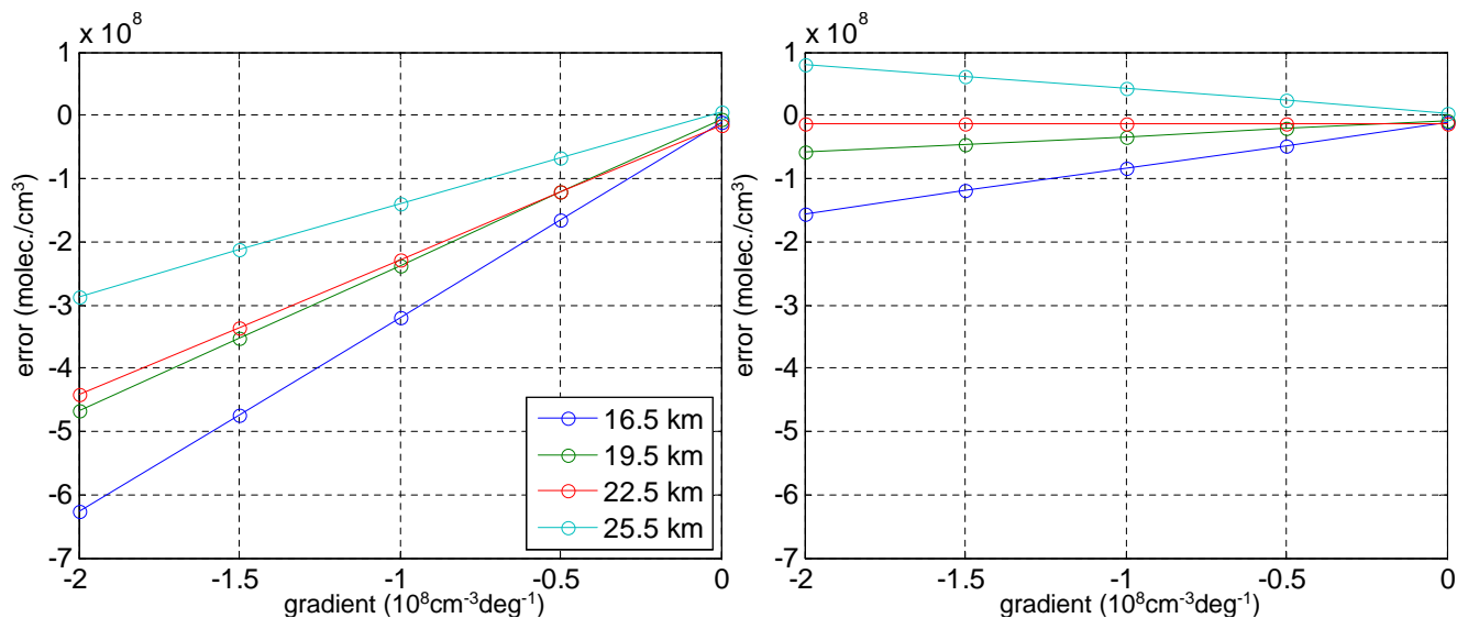
Fig. 13. The systematic error at 42° N in the retrieved number density of NO 2 as function of the simulated gradient strength between 40° and 50° for the 1-D (left) and 2-D (right) retrieval approach. On the x-axis the gradient strength at the peak of the simulated profile (28.5 km) is given. The colored lines display the difference to the true simulated values at the respective altitudes (16.5 km to 25.5 km, see legend).
