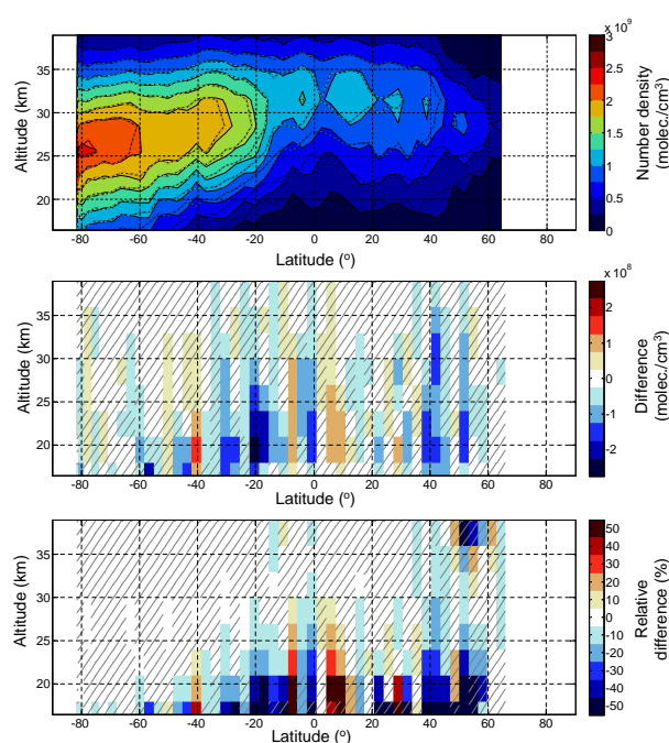
Fig. 5. Same as Fig. 4 but for orbit 35503.
