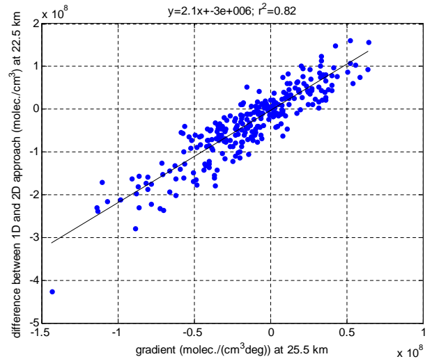
Fig. 8. Difference between the number density retrieved by the 1-D and 2-D approaches at 22.5 km as function of the horizontal gradient of the number density at 25.5 km as observed for the 2-D retrieval for all measurements of the full limb orbits on 14 December 2008. Also shown is the line of the best fit to the observed differences. Equation for the line of the best fit and squared correlation coefficient r^2 are provided in the title.
