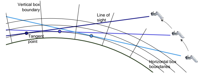
Fig. 2. Definition of the horizontal model space for the 2-D retrieval with respect to the tangent points of the scanning sequences. For illustration purposes, the LOS of only one measurement (for the same TH) per scanning sequence is shown.
