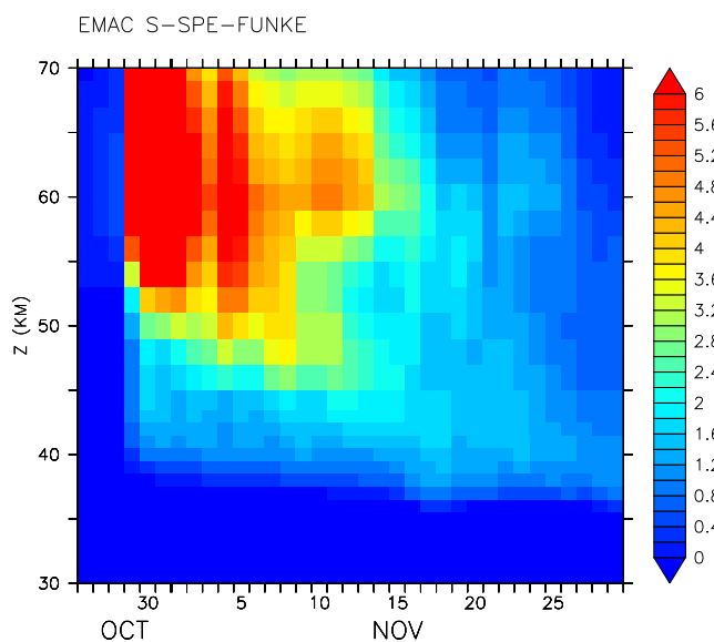
Fig. 6. N 2 O change (ppbv) in EMAC simulation S-SPE-FUNKE with respect to 26 October for 70–90° N.
