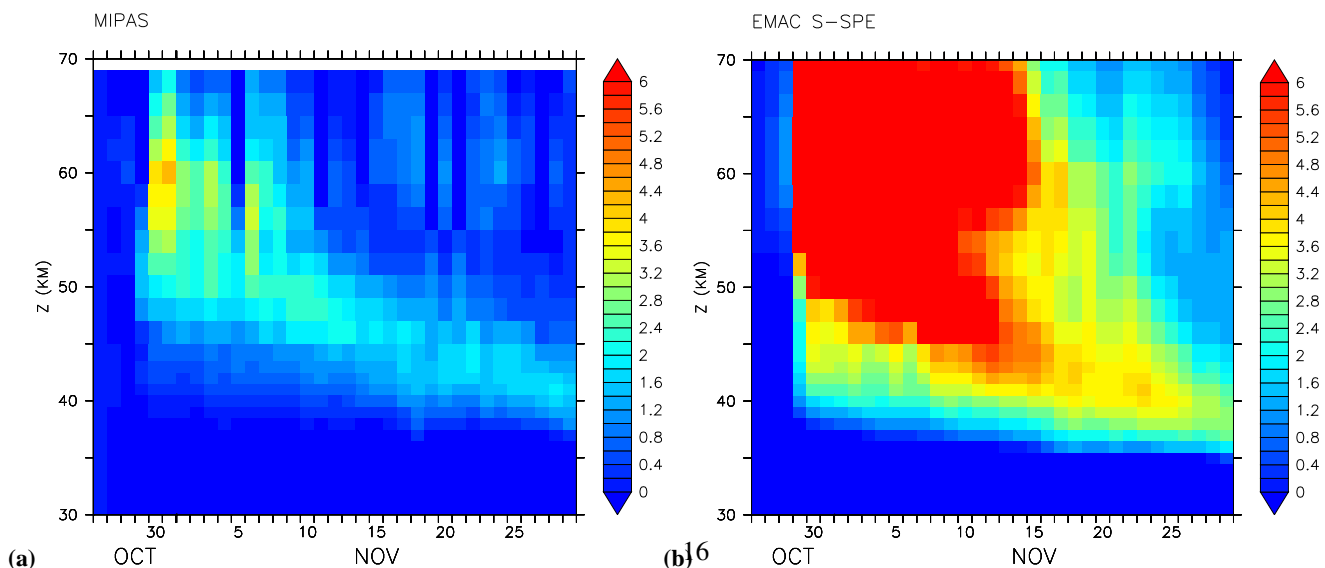
Fig. 5. Same as Fig. 4 but for N 2 O (ppbv).
