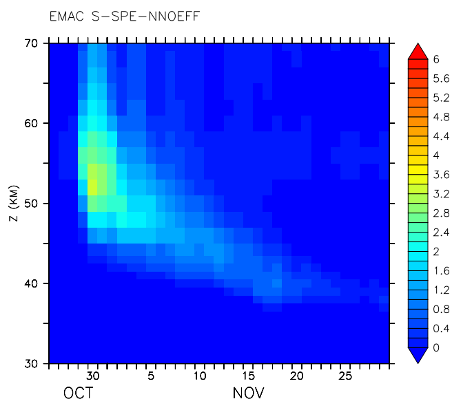
Fig. 11. Same as Fig. 10 but for \text{N}_2\text{O} changes (ppbv).
