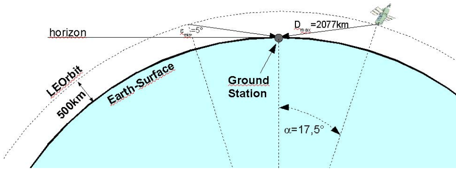
Figure 1: Link geometry of EO-Sat downlink with exemplary values (minimum elevation angle is 5^\circ , ground station at sea level), the maximum time fraction (with zenith-overflight) of one orbit’s contact to the ground station is 9,7%, the duration of one downlink is max. 9 minutes (from 5^\circ to zenith to 5^\circ elevation).
