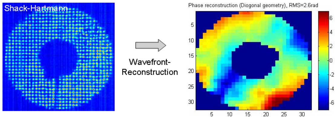
Figure 9: Typical image of the InGaAs Shack-Hartmann sensor with the reconstructed phase for a 400m link between two buildings. Both images show the central obscuration of the OGS-OP 40cm Cassegrain telescope.
