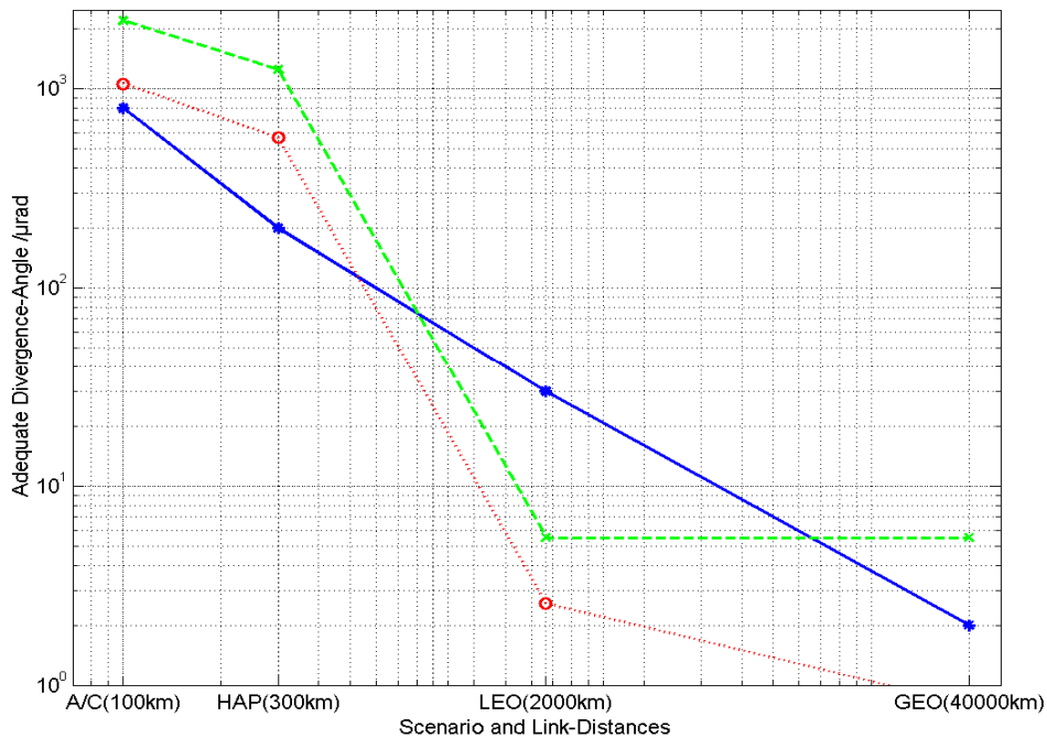
Figure 13: Relation between Link distance, remaining pointing error (dotted red), actual FWHM divergence angle (dashed green), and required FWHM beam divergence (solid blue). A typical set of parameters is used for link budget calculations here: 1.25Gbps, 100mW Tx-power, 0.4m Rx-aperture diameter, and receiver sensitivity is 70nW. See text above for explanations.
