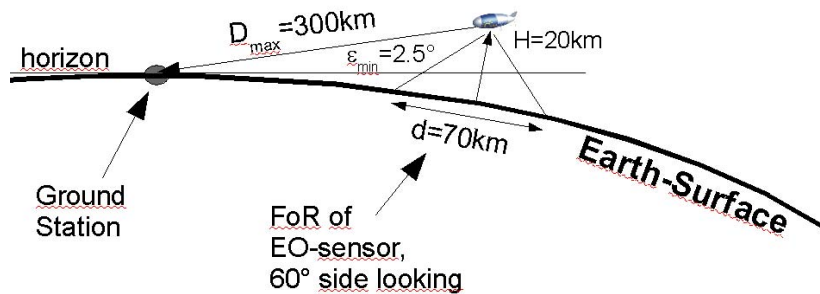
Figure 2: HAP downlink geometry
