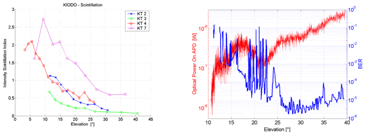
Figure 4: Examples of optical scintillation effects caused by IRT: Measured KIODO intensity scintillation index \sigma_I^2 over elevation at four different trials. One can observe scintillation saturation at low elevations and peaking between 5° and 10° (left). Received power and BER of KIODO trial #7 (right). The relatively high BER was caused by strong fading while the mean received power was more than sufficient. Clouds between 18° and 25° elevation caused power degradation and thus BER-surges, while the tracking lock was maintained.
