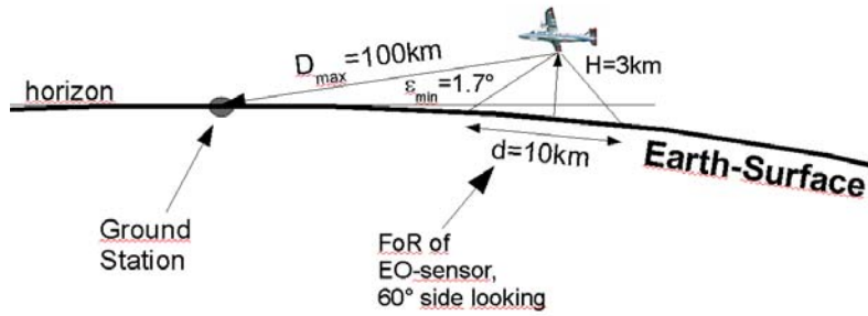
Figure 3: Optical aircraft downlink geometry
