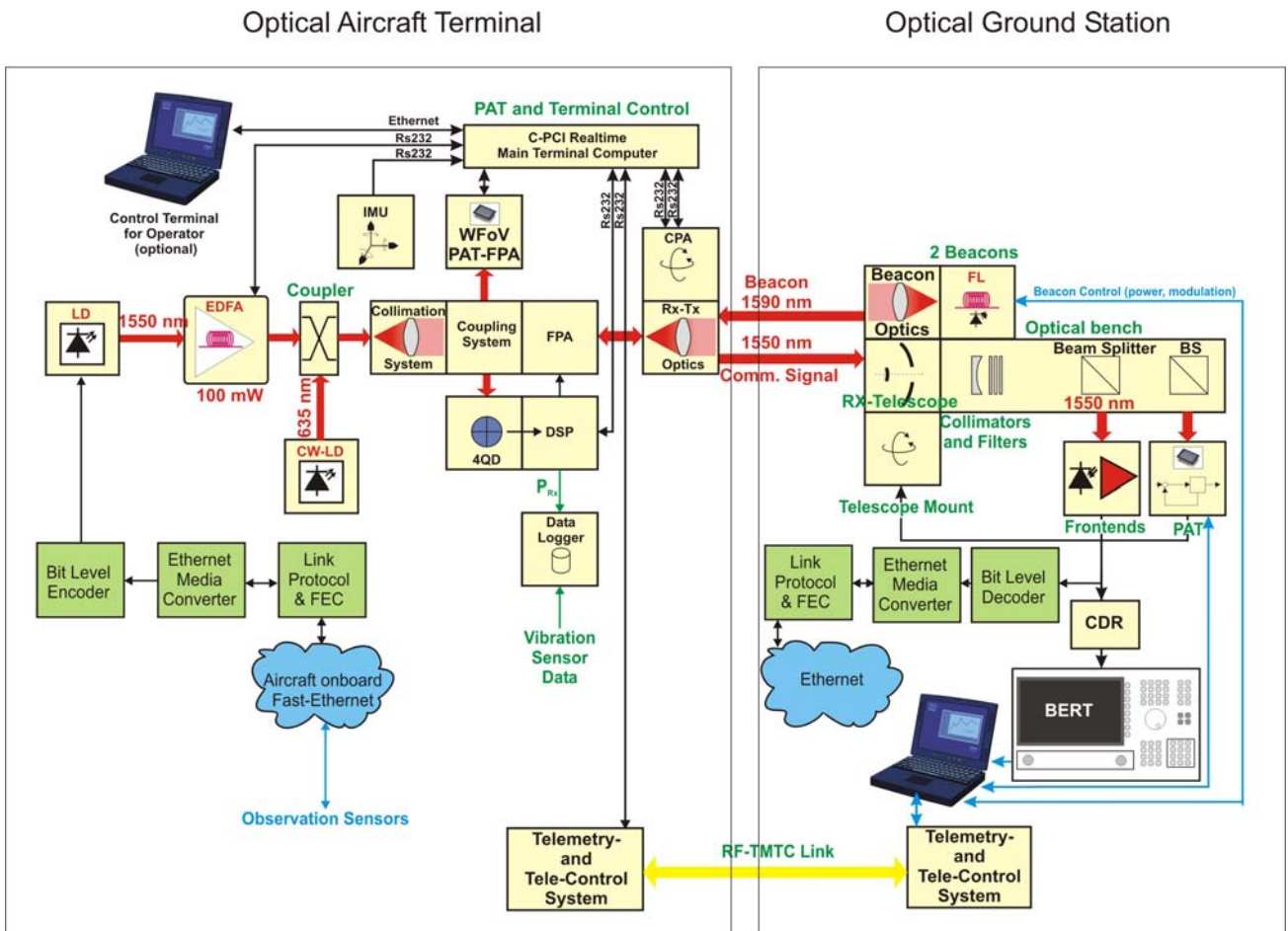
Figure 12: Schematic of the ARGOS system. In the left box the optical aircraft terminal setup can be seen and in the right the components of the OGS.
