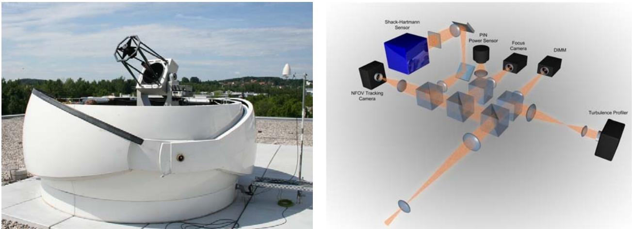
Figure 5: Optical Ground Station Oberpfaffenhofen (OGS-OP). Photograph of dome, mount, and telescope (left), optical path of the measurement devices (right).
