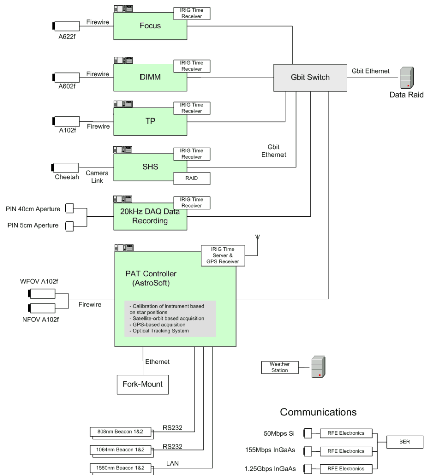
Figure 6: Functional Diagram of the OGS-OP – Atmospheric measurement instruments, PAT system, and communication systems.
