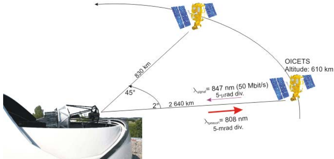
Figure 7: Overview of the KIODO downlink scenario
