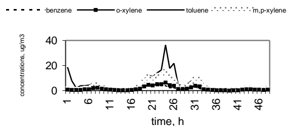
Figure 1. Diurnal variation of BTX concentrations in Wroclaw, September, 18-19, 2006.
