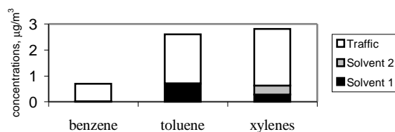
Figure 2. The monthly average mean of BTX concentrations and the concentrations calculated by the CMB model for traffic and solvent use emissions.
