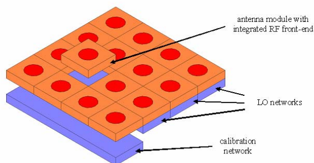
Fig. 1 Schematic of antenna array
