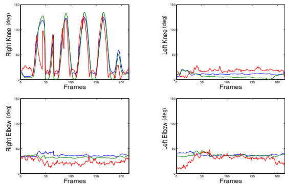
Fig. 2. Plots of four joint angles (deg) during the right knee flexion-extension. We compare the Kinect skeleton (red curves) and the WIMU orientations (blue curves) to the Vicon system (green curves) as a ground truth reference.
