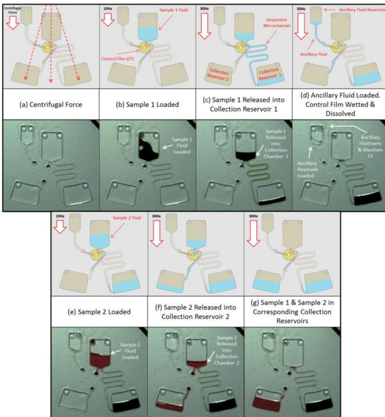
Figure 5: Co-located valving applied to selective fluid routing. (a) Basic structure. (b-c) Loading of sample and its routing past a DF film, recessed in a dead-end channel, and into collection reservoir 1. This can be repeated for multiple liquid elements. (d) Loading of ancillary liquid. This is routed past the DF and dissolves it ‘from below’, thus opening a route to collection reservoir 2. (e-g) Liquid added to the main reservoir is now routed to the collection reservoir 2.
