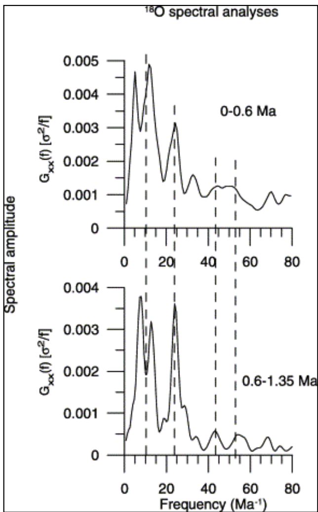
Fig. 6. Spectral analyses using SPECTRUM ([Schulz and Stettger, 1997]) of the \delta^{18}\text{O} results. The oxygen isotopes do not show as marked a difference between the dominating 100-kyr (10/Ma) and 40-kyr (25/Ma) cyclicity as do the carbonate results (Fig. 5) for the periods 0–0.6 Ma and 0.6–1.35 Ma respectively.
