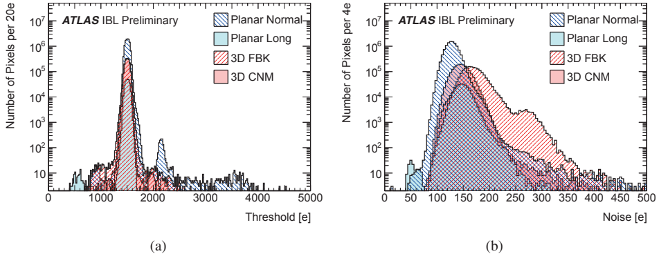
Figure 4.15: (a) Threshold and (b) noise distributions after tuning all pixels to a target threshold of 1500 e^- at -12^\circ C module temperature for 18 production staves [45].
