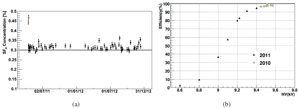
Figure 5.3: (a) SF 6 concentration in the CMS RPC fresh mixture. The red dots are the data of April 2011 when a drift in the MFC flow was detected. (b) Mean efficiency of some CMS RPC detectors as a function of the applied voltage in 2010 and 2011. The 2011 data correspond to an increase of SF 6 (from 0.30% to 0.45%): an increase of about 120 V is necessary to operate at the same operation conditions.
