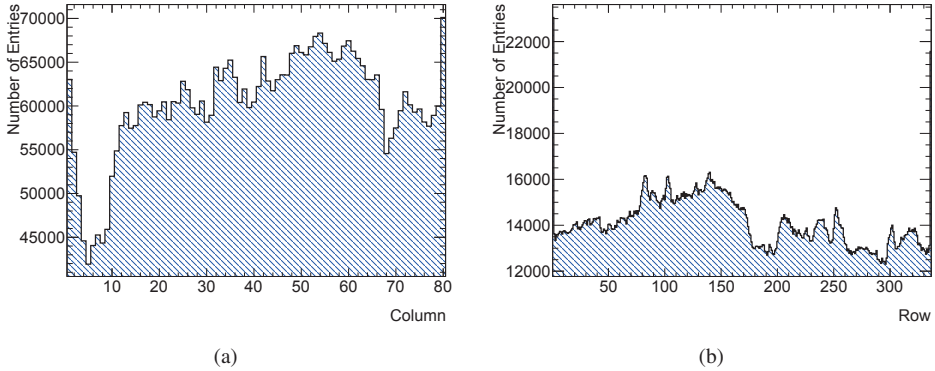
Figure 4.21: (a) Projection of the occupancy plot on the columns and (b) projection of the occupancy plot on the rows for a FBK sensor on ST11 irradiated with ^{90}\text{Sr} at 22^\circ\text{C} with a 3000\text{ e}^- threshold and 10 BCs ToT at 16000\text{ e}^- tuning. The number of entries is not uniform distributed because of SMD components, however it is visible a higher number of entries in both external columns and rows.
