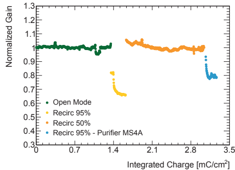
Figure 6.29: Normalized gain as a function of integrated charge for the triple-GEM detector operated with Ar/CO 2 /CF 4 (45/15/40) gas mixture with different recirculation rates with and without the use of purifier in the gas system.
