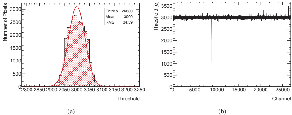
Figure 4.11: Threshold distribution of a FE-I4 chip (A1-1- in ST18) after a successful tuning procedure for reference threshold of 3000 e^- at 22^\circ\text{C} . (a) Fit of the threshold values and (b) threshold values as a function of pixel channels, where channel number is calculated as (\text{row}+\text{col})\times 336 .
