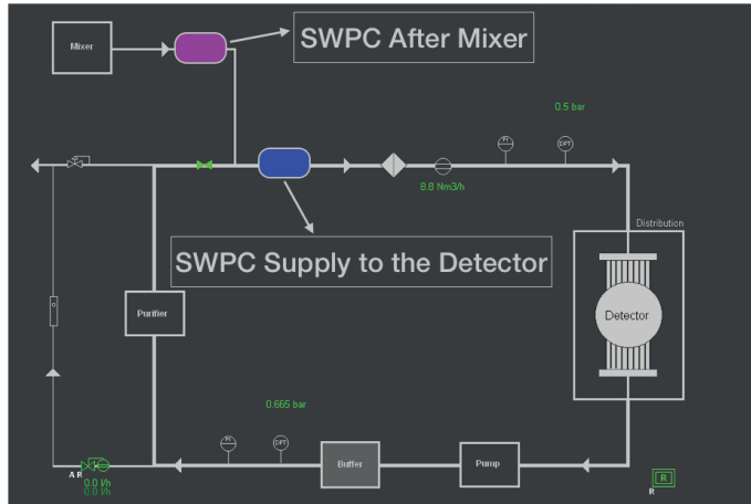
Figure 6.13: Schematic view of the CSC gas system. The position of the two SWPCs is indicated in the schematic. SWPC “After Mixer” is located right after the mixer to analyze the fresh gas mixture injected into the gas system while SWPC “Supply to the Detector” is located after the purifier and the fresh mixture line to analyze the gas that is directly injected into the detector.
