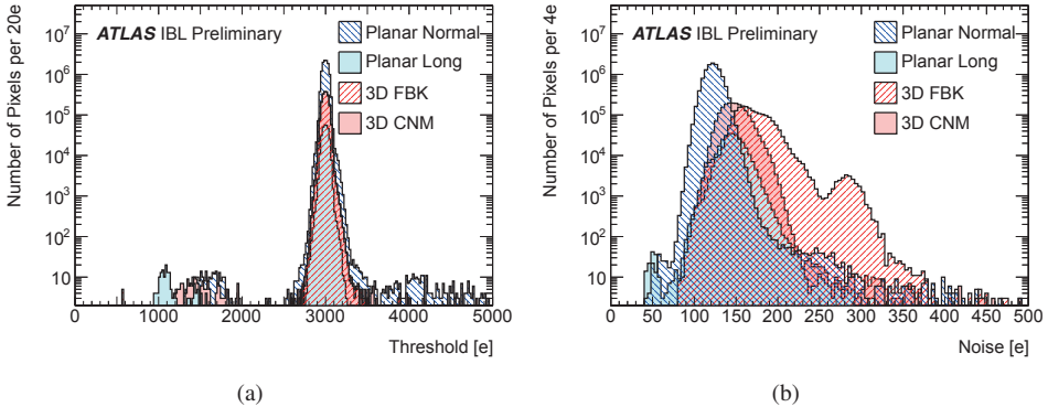
Figure 4.14: (a) Threshold and (b) noise distributions after tuning all pixels to a target threshold of 3000 e^- at 22^\circ\text{C} module temperature for 18 production staves [45].
