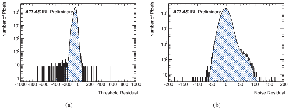
Figure 4.9: Pixel by pixel (a) threshold and (b) noise residuals between the stave loading and stave QA sites. Only eight staves are used for this comparison [45].
