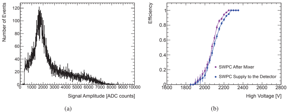
Figure 6.14: (a) Pulse-height spectrum of a SWPC irradiated with a ^{109}\text{Cd} radioactive source. The 22 eV gamma peak is clearly visible. (b) Efficiency of the two SWPCs used for the gas monitoring in the CMS CSC gas system. The names “After mixer” and “Supply to the Detector” refer to their position in the gas system.
