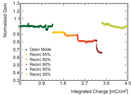
Figure 6.26: Normalized gain as a function of integrated charge for the triple-GEM detector operated with Ar/CO 2 /CF 4 (45/15/40) gas mixture during different rates of recirculated gas. The gain has been corrected for temperature and pressure variations using the parameters of the fit obtained in Figure 6.22(b).
