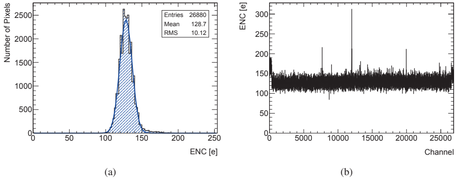
Figure 4.12: Noise distribution of a planar module (A1-1- in ST18) after a successful tuning procedure for reference threshold of 3000\text{ e}^- at 22^\circ\text{C} .
