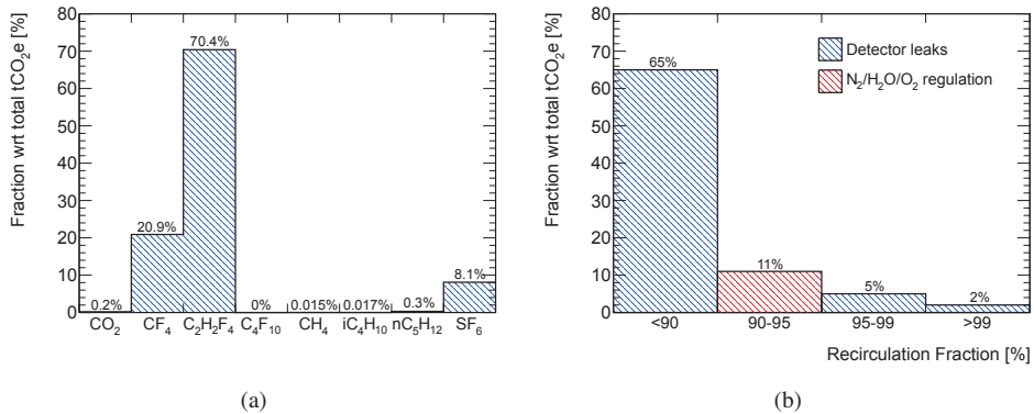
Figure 5.9: (a) Relative contribution in terms of CO 2 equivalent from different gases used for particle physics detection at CERN. The dominant contribution is due to the C 2 H 2 F 4 used by the large ATLAS and CMS RPC systems. (b) Fraction with respect to the total of the equivalent CO 2 emission for the gaseous detectors operated with different recirculation efficiencies. Only a low contribution is due to the need to adjust the N 2 concentration in the gas mixture (in red).
