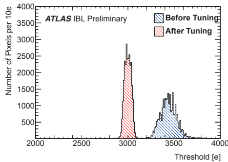
Figure 4.10: Threshold distribution of pixels before and after tuning for an IBL chip for 3000 e^- threshold tuning at 22^\circ\text{C} powering group temperature [45].
