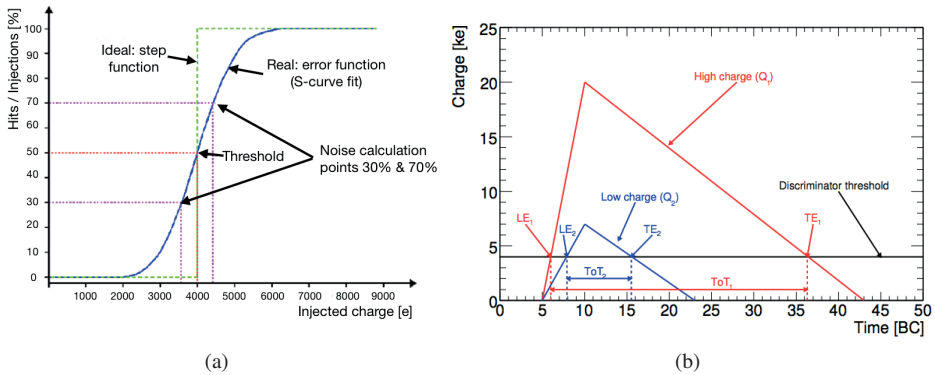
Figure 4.7: (a) Schematics of an example of S-curve with the method to select the threshold and noise. (b) Overview of the ToT method to defined the charge [50].
