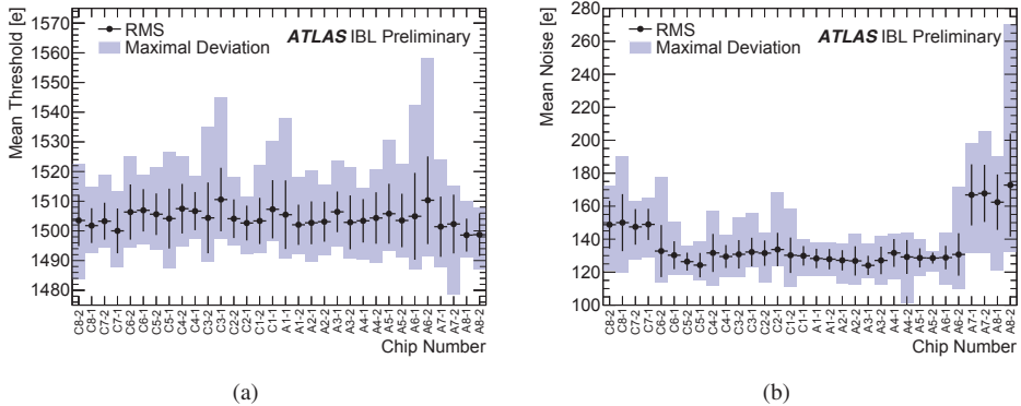
Figure 4.16: Average (a) threshold and (b) threshold noise distributions for all 18 production staves as a function of chip number for the 1500 e^- threshold tuning at -12^\circ C . The plots show, for each chip position on the stove, the mean and scatter of the 18 data points (one from each stove). The error bars show the RMS spread, while the solid boxes show the minimum and maximum values [45].
