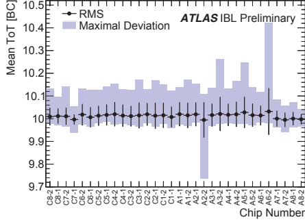
Figure 4.18: Average ToT distribution as a function of chip number for all 18 production staves. The pixels were tuned to 1500 e^- target threshold and to a 10 ToT target response for 16000 e^- at -12^\circ C [45].
