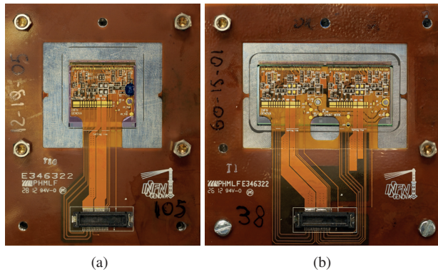
Figure 3.9: Photo of a dressed IBL (a) single chip and (b) double chip modules. The flex extension is present to allow testing the module prior to its loading on the stave.
