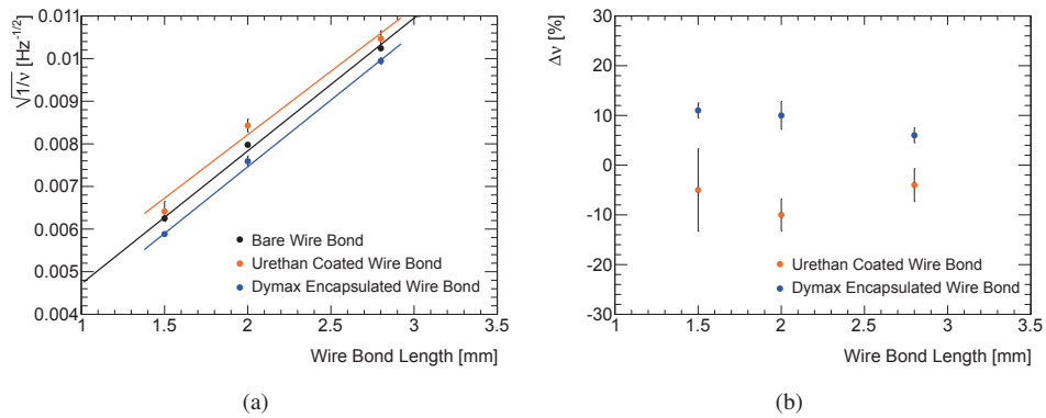
Figure 4.36: (a) Resonance frequency as a function of wire bond length for bare, Urethan coated and Dymax encapsulated wire bond. (b) Resonance frequency shift after the application of urethan or Dymax to bare wirebonds.
