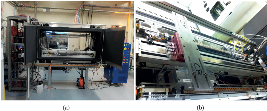
Figure 4.3: Stave QA test stand pictures showing the (a) outside and (b) inside of the environmental box.
