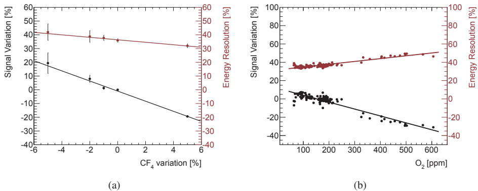
Figure 6.7: (a) Pulse charge spectrum mean and energy resolution for SWPC as a function of CF_4 variation considering Ar/CO_2/CF_4 (45/15/40) as the base gas mixture ( CF_4 variation equal to zero) and at constant electric field. (b) Signal variation and energy resolution of SWPC spectrum as a function of O_2 concentration for Ar/CO_2/CF_4 (55/40/5) gas mixture considering 150 ppm as the reference O_2 concentration.
