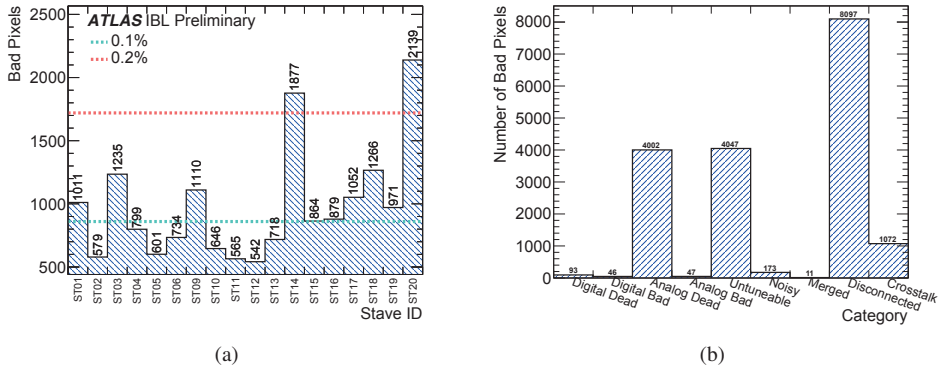
Figure 4.30: Number of bad pixels (a) per stave and (b) for 18 production staves.
