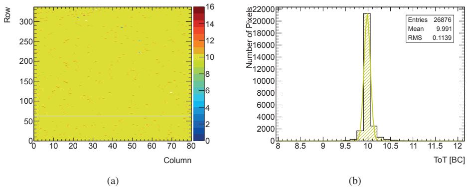
Figure 4.13: ToT scan response to 16000\text{ e}^- injected for a FE-I4 chip (A1-1 in ST18) after a successful tuning procedure for reference threshold of 3000\text{ e}^- and ToT tuned to 10 BC for a reference mip charge of 16000\text{ e}^- at 22^\circ\text{C} . (a) ToT scan 2D map for all FE-I4 channels and (b) fit of the ToT values.
