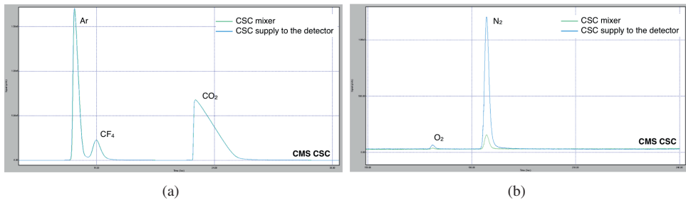
Figure 5.2: (a) Gas chromatograms of the CMS CSC gas mixture in two analysis points. “CSC mixer” is the GC analysis of the gas mixture after the mixer while “CSC supply to the detector” is the GC analysis of the gas mixture sent to the detector after purification and the addition of a small percentage of fresh gas. (b) The “CSC supply to the detector” contains a higher quantity of both components coming from the CSC permeability to Air.
