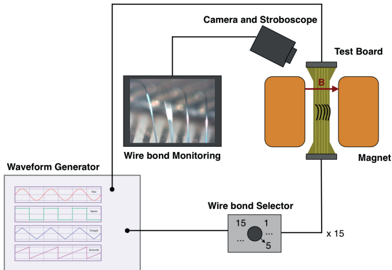
Figure 4.32: Schematic view of the experimental set-up used to test IBL-like wire bonds in 2 T magnetic field.
