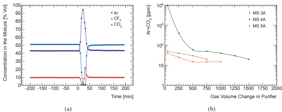
Figure 5.8: (a) \text{CO}_2 absorption at the beginning of a purifier cycle. It is evident how the gas mixture ratios are completely destabilized during this phase. (b) Ar release during the first operation phase of a purifier. Ar is present in the material since it is used during the regeneration process.
