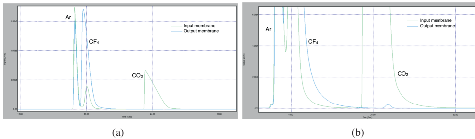
Figure 5.11: (a) Comparison of the gas chromatograms at the input (green line) and output (blue line) of the membrane module. Most of the \text{CO}_2 has been absorbed. The mixture composition changes from \text{CO}_2/\text{Ar}/\text{CF}_4 (50/40/10) to \text{CO}_2/\text{Ar}/\text{CF}_4 (<1/60/40). (b) A zoomed view of the \text{CO}_2 peak: a small concentration of \text{CO}_2 is still present (< 1%).
