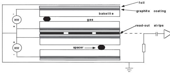
Figure 6.30: Cross-sectional view of a double gap RPC.
