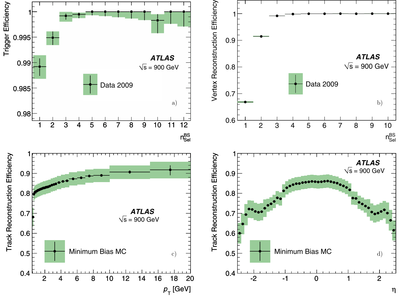
Fig. 2. Trigger (a) and vertex-reconstruction (b) efficiencies as a function of the variable n_{\text{Sel}}^{\text{BS}} defined in Section 4; track-reconstruction efficiency as a function of p_T (c) and of \eta (d). The vertical bars represent the statistical uncertainty, while the shaded areas represent the statistical and systematic uncertainties added in quadrature. The two bottom panels were derived from the PYTHIA ATLAS MC09 sample.
