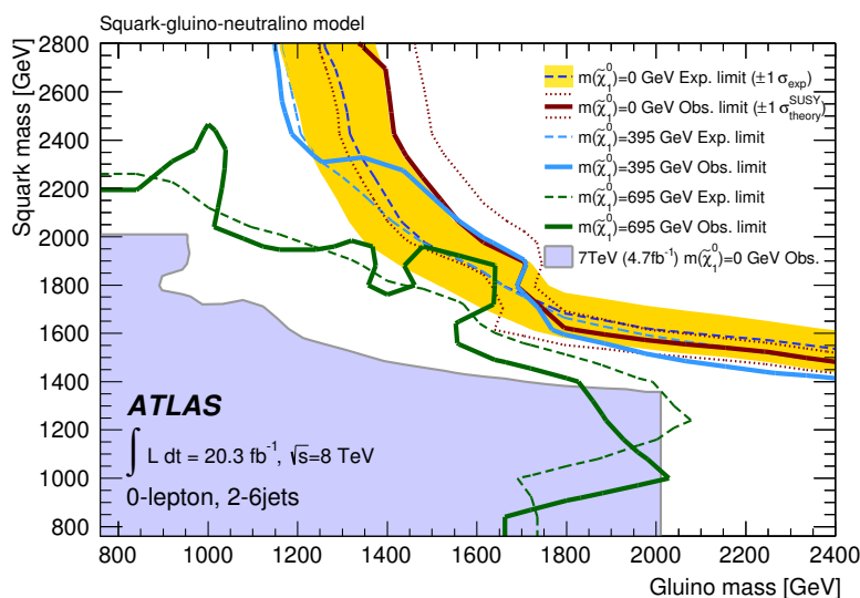
Figure 9. Exclusion limits for a simplified phenomenological MSSM scenario with only strong production of gluinos and first- and second-generation squarks (of common mass), with direct decays to quarks and lightest neutralinos. Three values of the lightest neutralino mass are considered: m_{\tilde{\chi}_1^0} = 0, 395 GeV and 695 GeV. Exclusion limits are obtained by using the signal region with the best expected sensitivity at each point. The dashed lines show the expected limits at 95% CL, with the light (yellow) band indicating the 1\sigma experimental and background-only theory uncertainties on the m_{\tilde{\chi}_1^0} = 0 limit. Observed limits are indicated by solid curves. The dotted lines represent the m_{\tilde{\chi}_1^0} = 0 observed limits obtained by varying the signal cross-section by the renormalisation and factorisation scale and PDF uncertainties. Previous results for m_{\tilde{\chi}_1^0} = 0 from ATLAS at 7 TeV [16] are represented by the shaded (light blue) area. Results at 7 TeV are valid for squark or gluino masses below 2000 GeV, the mass range studied for that analysis.
