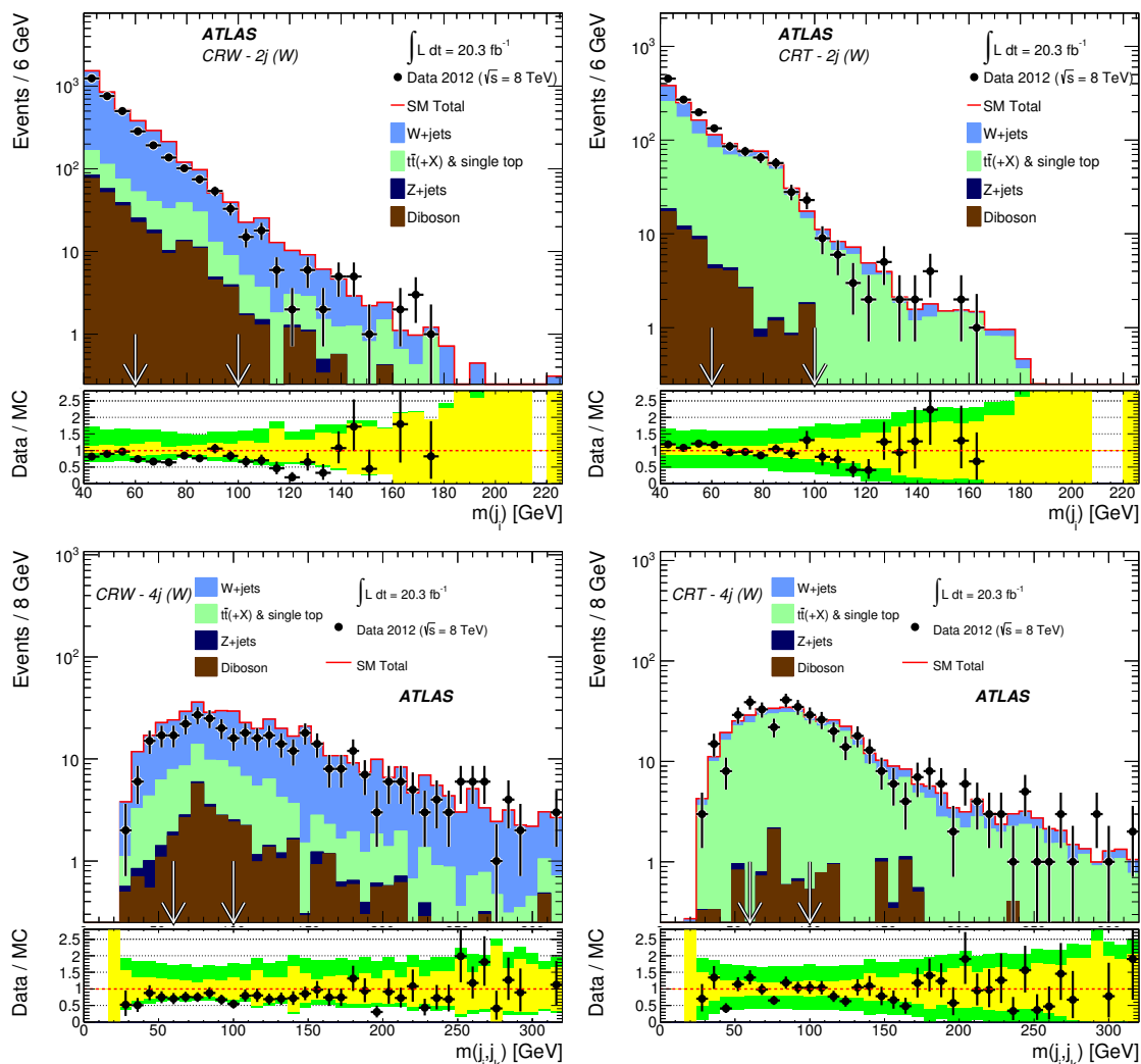
Figure 2. Observed jet (top) or dijet (bottom) mass distributions for the CRW (left) and CRT (right) selections for the 2jW (top) and 4jW (bottom) signal regions. In the case of the dijet mass distributions for SR 4jW (bottom), events are required to possess at least one unresolved W candidate, with the dijet mass calculated from jets excluding the unresolved W candidate. With the exception of the multi-jet background (which is estimated using the data-driven technique described in the text), the histograms denote the MC background expectations, normalised to cross-section times integrated luminosity. In the lower panels the light (yellow) error bands denote the experimental systematic and MC statistical uncertainties, while the medium dark (green) bands include also the theoretical modelling uncertainty.
