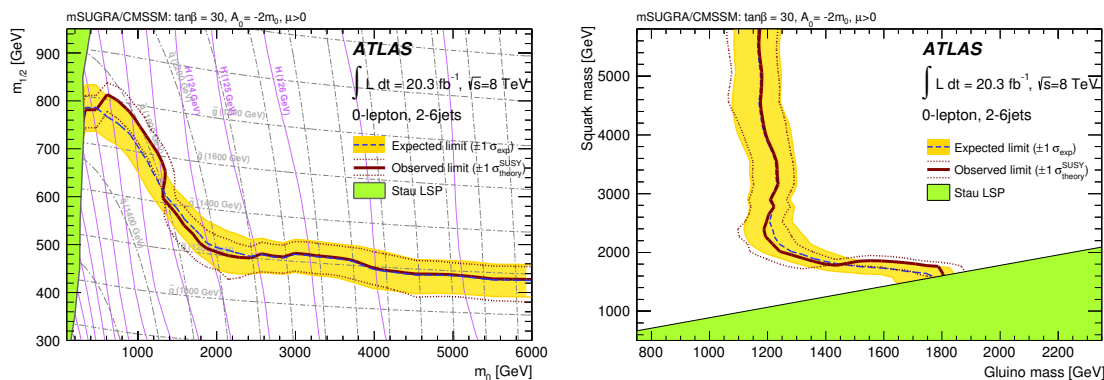
Figure 8. Exclusion limits for mSUGRA/CMSSM models with \tan\beta = 30 , A_0 = -2m_0 and \mu > 0 presented (left) in the (m_0, m_{1/2}) -plane and (right) in the (m_{\tilde{g}}, m_{\tilde{q}}) -plane. Exclusion limits are obtained by using the signal region with the best expected sensitivity at each point. The blue dashed lines show the expected limits at 95% CL, with the light (yellow) bands indicating the 1\sigma excursions due to experimental and background-only theory uncertainties. Observed limits are indicated by medium dark (maroon) curves, where the solid contour represents the nominal limit, and the dotted lines are obtained by varying the signal cross-section by the renormalisation and factorisation scale and PDF uncertainties.
