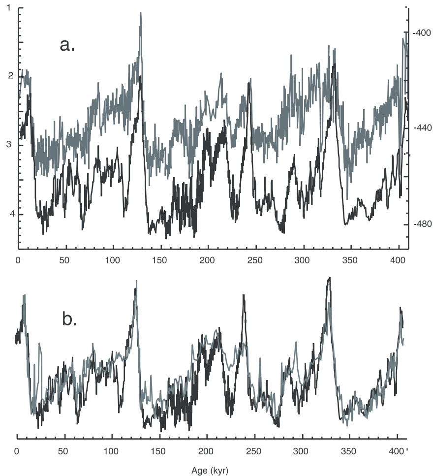
Figure 6. (a) Comparison between the Vostok deuterium record (taken from Vimeux et al. [2001]) and G. bulloides \delta^{18}O (gray) from ODP Site 1089 over four glacial cycles. The Vostok chronology was adjusted iteratively (and subjectively) to achieve maximum correlation with the Site 1089 record. (b) One independent, but lower-resolution cross-check on this synchronization comes from the \delta^{18}O record of TN057-6 (gray) [from Hodell et al. , 2000].
