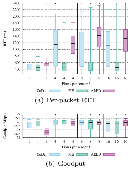
Figure 10: Uplink's Per-packet RTT and TCP goodput at the bottleneck link (per 5-sec intervals). 802.11 mixed traffic scenario for 4 senders, RTT_{base}=100 ms and target\_delay=5 ms.
