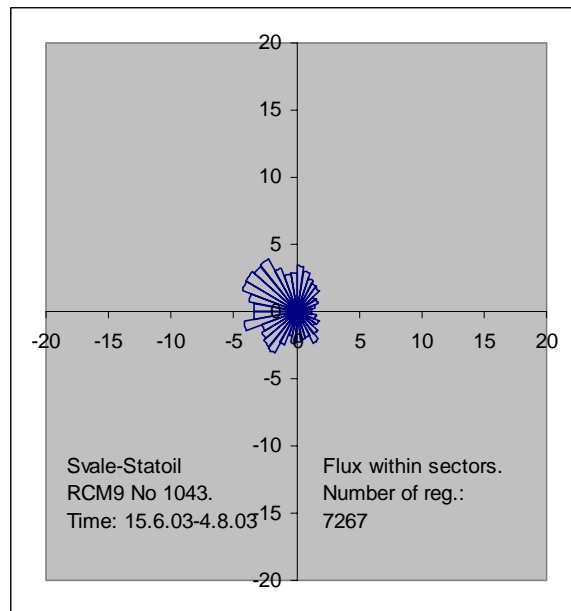
Figure 9. Directional distribution of mean current speed and flux, within sectors for the RCM9, ca 2m above the bottom.
