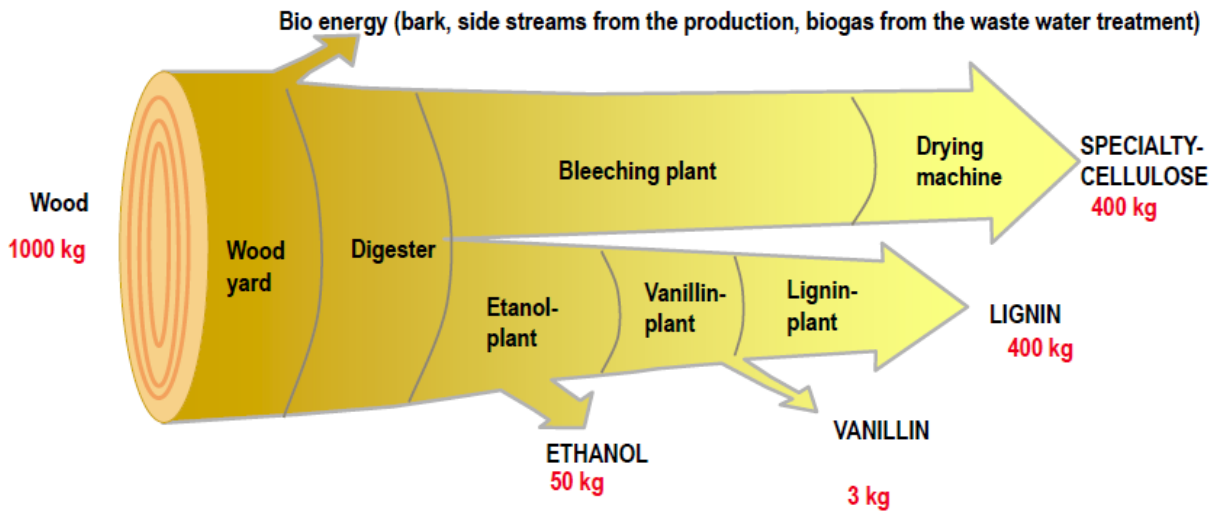
Figure 2: Process diagram for Borregaard Industries - overview
