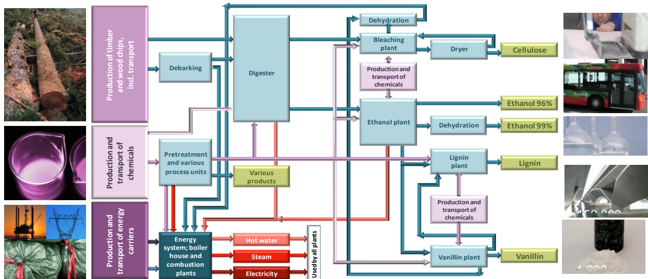
Figure 3: Process diagram for Borregaard Sarpsborg
