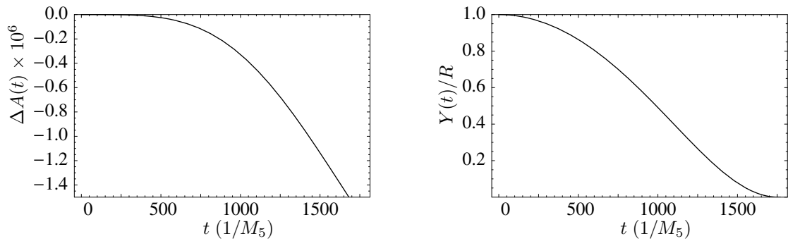
Figure 6.4: Numerical results with parabolic potential and constant B(t) and C(t) . Parameter values \alpha = 100M_5 , \beta = 1/1000 \times M_5 .
