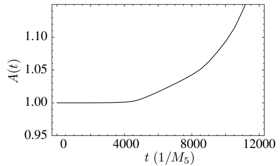
(b) A(t) climbs as the bulk brane gets close to the visible brane.
