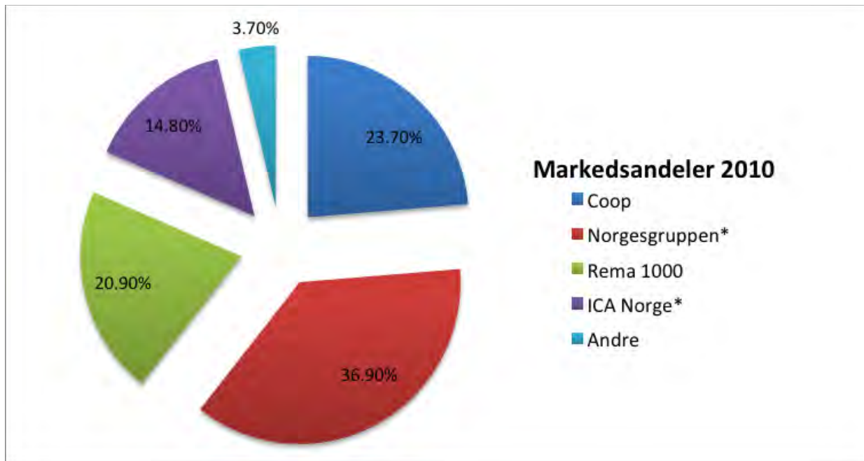
Figur 6: Markedsandeler 2010
