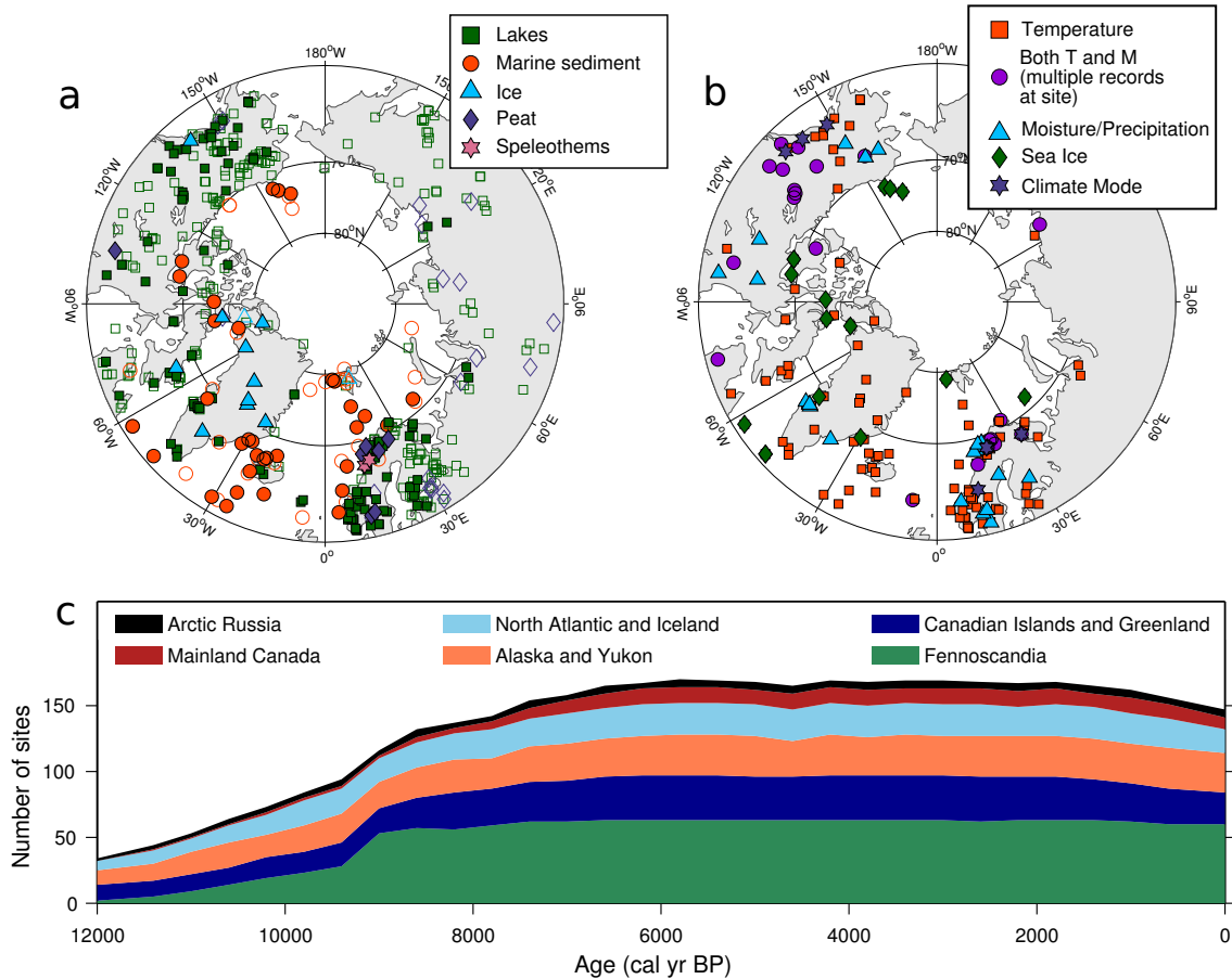
Figure 2. Location of proxy records in this database. (a) Sites that meet the criteria for inclusion in this database (solid symbols) and those that did not (open symbols) plotted by material/archive type. (b) Sites that meet the criteria plotted by broadly categorized climate variables ( T and M : temperature and moisture variables of all types, respectively). (c) Number of sites showing the time period they cover and subdivided by region. Some sites have more than one time series representing different climate variables. Information about each site is listed in Table 1 (accepted records) and Supplement Table S1 (excluded records).
