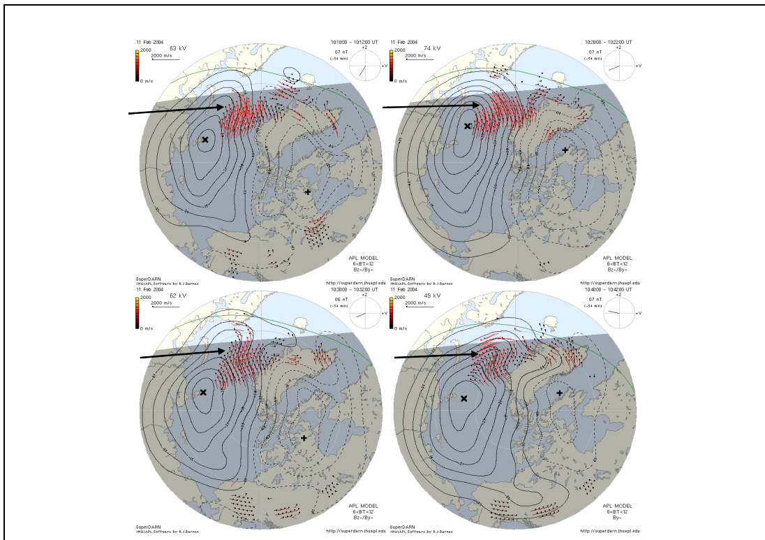
Figure 4.16: SuperDARN data with an adapted field model.
