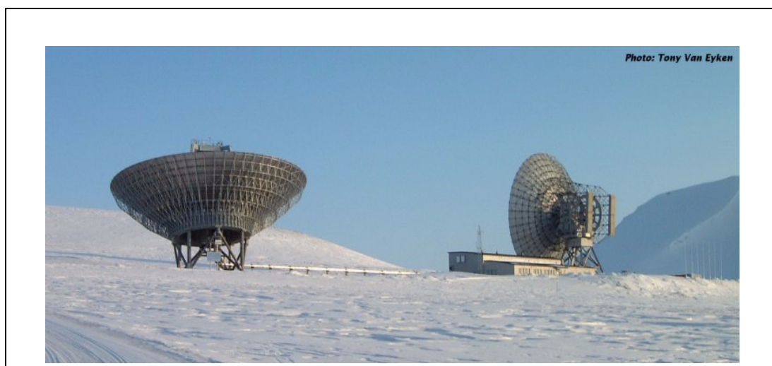
Figure 3.7: The 32m and 42m parabolic dish situated outside Longyearbyen, Svalbard (photographed by Tony Van Eyken).
