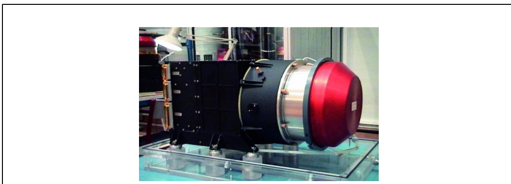
Figure 3.2: One of the four CIS-experiments developed for the Cluster mission.
