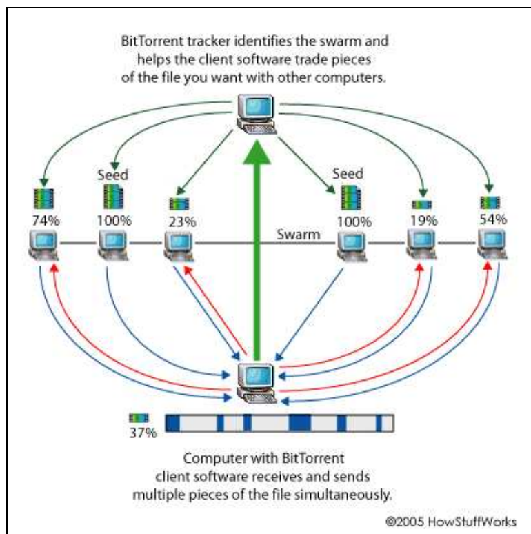
Figure 2.3: How a BitTorrent swarm works. The client receives segments from the other peers and sends information back to the tracker. Taken from[1].
