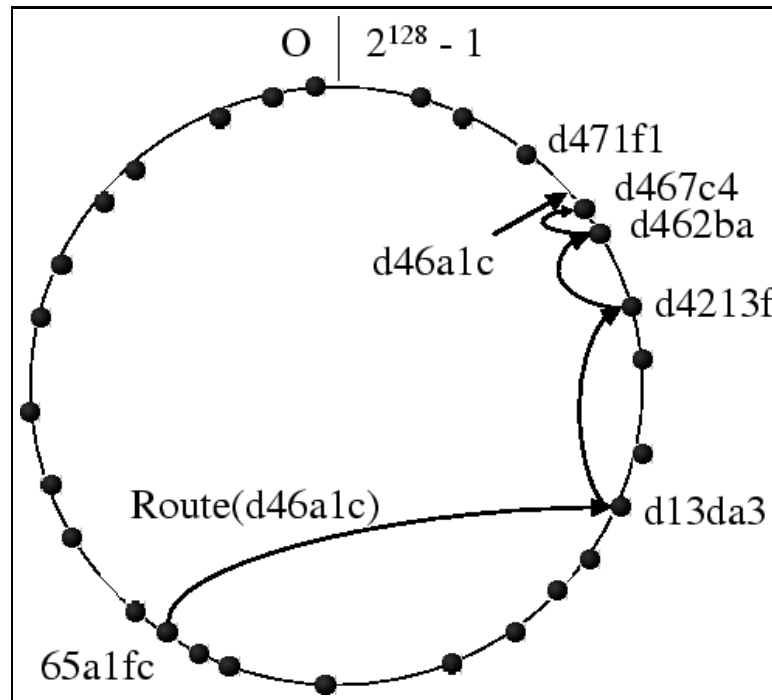
Figure 2.4: Routing a message from node 65a1fc with key d46a1c . The dots depict live nodes in Pastry's circular name space. From [2].
