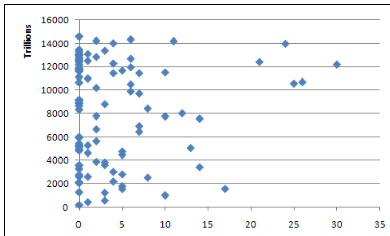
Figure 5.3: 400 mirrors spread out over 100 nodes using the property id-base model with 4 service types and 2 properties. Y-axis shows the node id in 10 base. X-axis is the number of service mirrors a node is holding.
