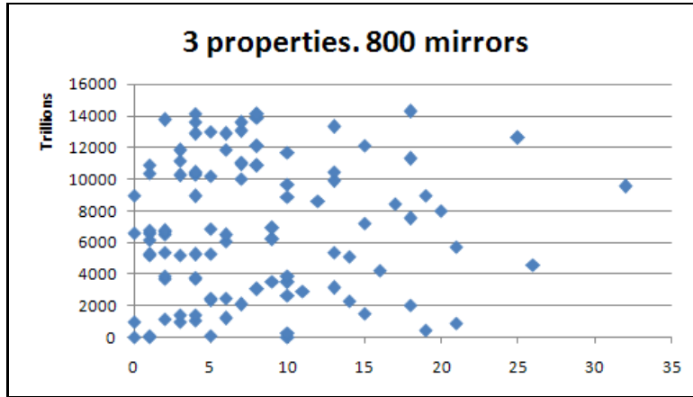
Figure 5.2: 800 different mirrors spread out over 100 nodes using the property id-base model. Y-axis shows the node id in 10 base. X-axis is the number of service mirrors a node is holding.
