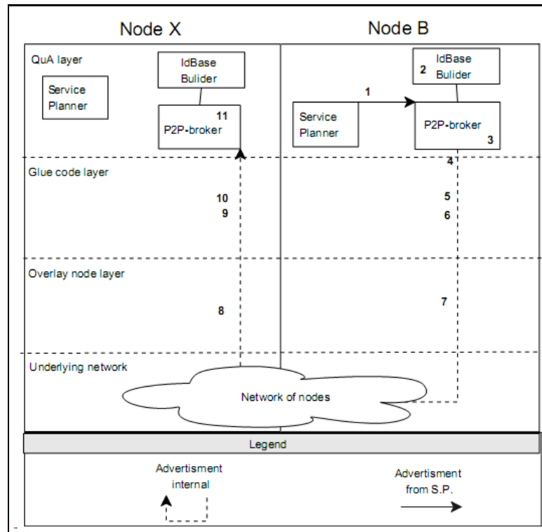
Figure 3.1: Layer responsibility when a service mirror is advertised. Taken from [4].
