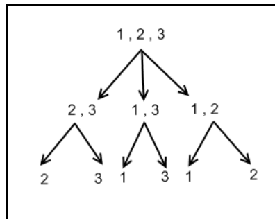
Figure 3.3: All possible unordered combinations with the numbers 1, 2 and 3 with the use of a non-optimized recursive method.
