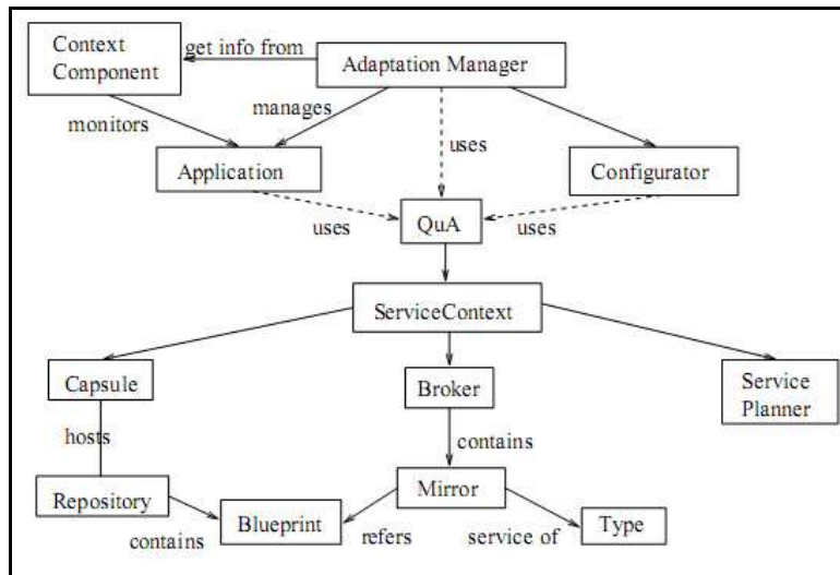
Figure 2.5: The QuA middleware. Taken from [3]
