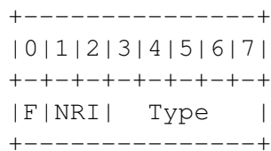
Figure 2.3: The NAL unit header as defined by RFC 3984 [7]
