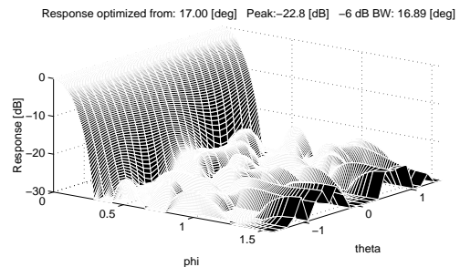
Figure 4. Beampattern for weighted, optimally thinned layout (62 elements out of 112)
