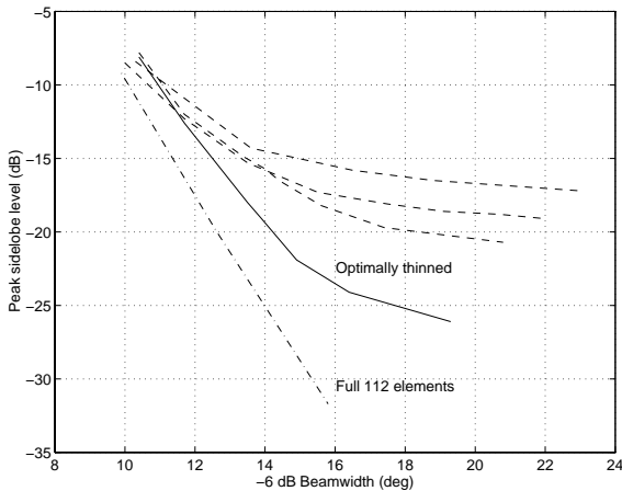
Figure 2. Sidelobe level as a function of beamwidth for several weight-optimized uniform sidelobe cases: 112 element full array (dash-dot line) and three realizations of random thinning to 64 elements (dashed lines). The best result is obtained for a layout-optimized 62 element thinning (solid line).
