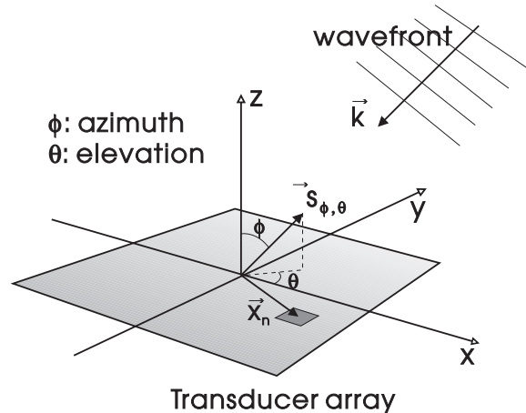
Figure 1. A 2D planar array with coordinate system.
