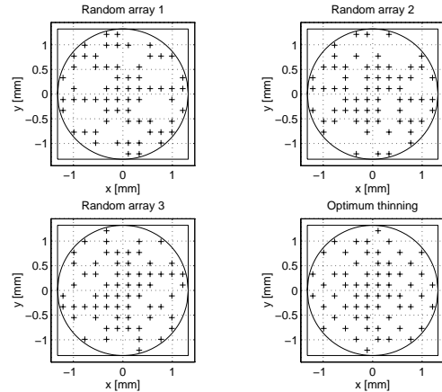
Figure 3. Element layouts for 112 element full array thinned to three different random 64 element layouts and a 62 element optimized layout. The random arrays are sorted according to the peak sidelobe level in Fig. 2 with Random 1 having the highest peak sidelobe level for large beamwidths.
