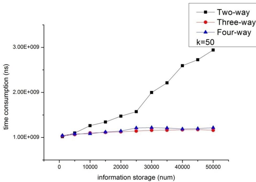
Figure 5.8: Evaluation result curve (k=50)
