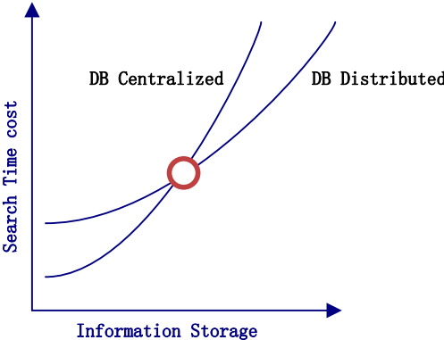
Figure 3.7: Experiment hypothesis
